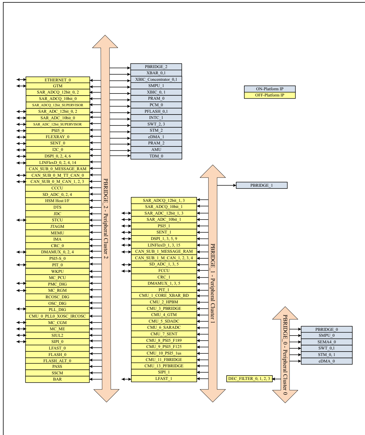
Figure 2. Periphery allocation
