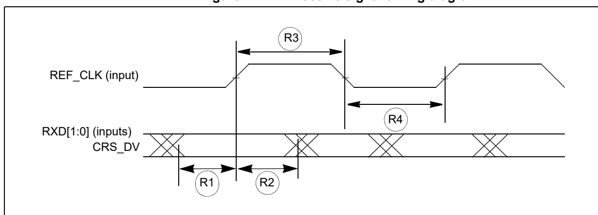
Figure 41. RMII receive signal timing diagram
