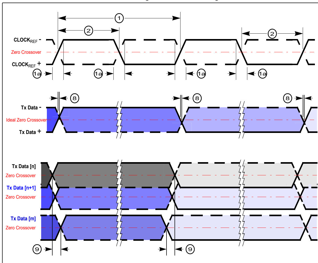
Figure 22. Aurora timings
