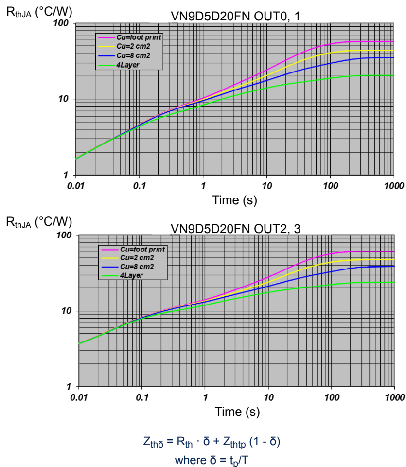
Figure 51. Thermal fitting model
