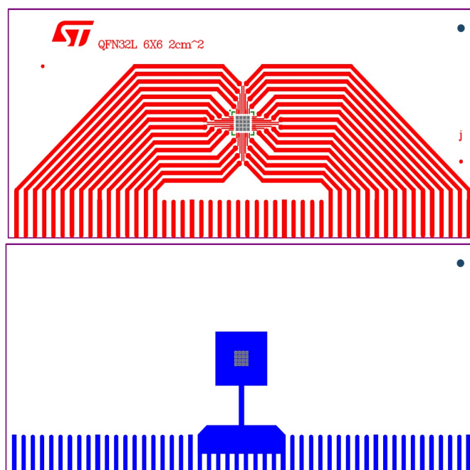
Figure 46. QFN 6x6 PCB 2 cm 2
