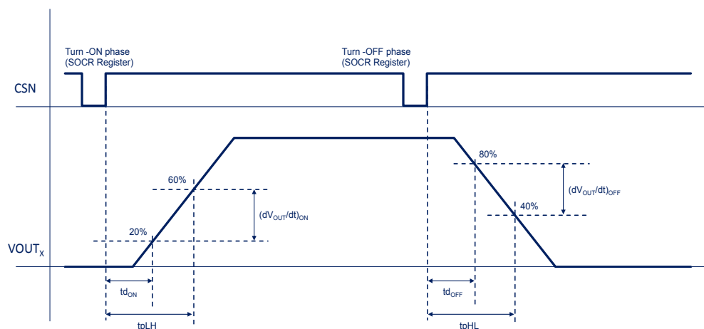
Figure 33. Switching characteristics
