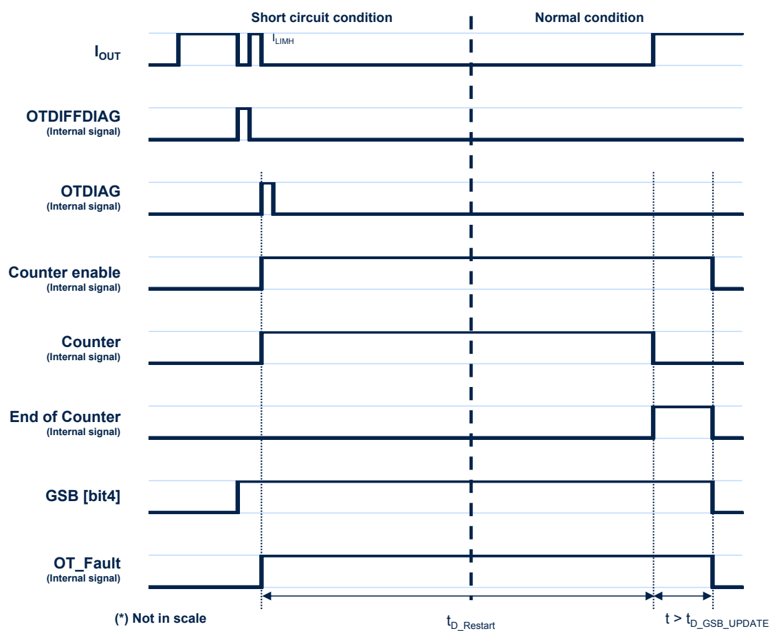
Figure 35. Normal mode - Short circuit – PBW > t_{D\_Restart}
