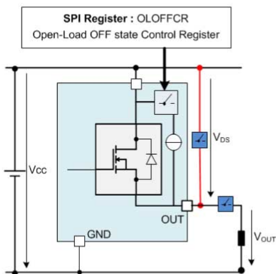
Figure 26. Open-load OFF-state detection
