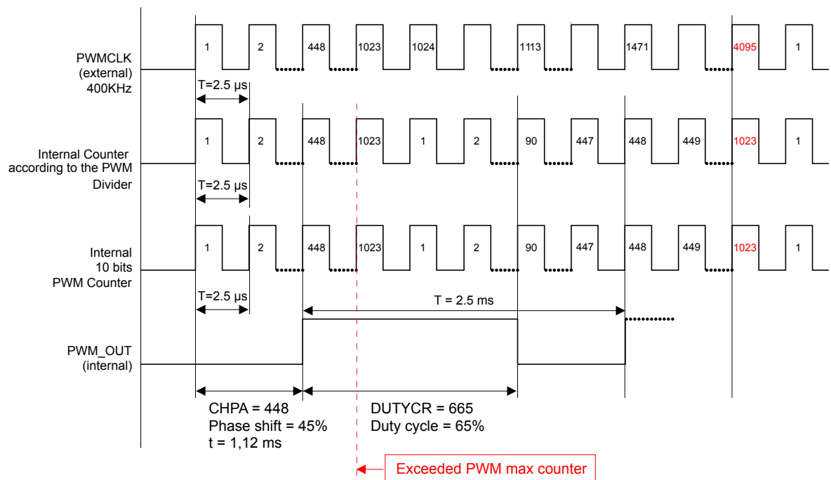
Figure 13. Resulting waveform 2
