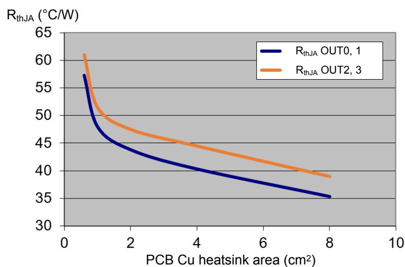
Figure 49. R_{thJA} vs PCB copper area in open box free air conditions
