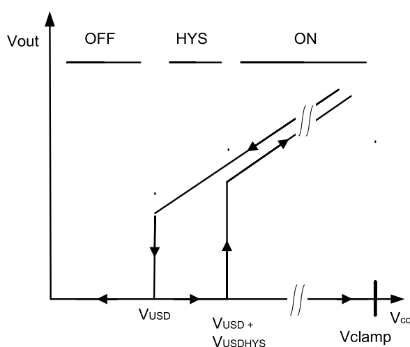
Figure 5. Undervoltage shutdown
