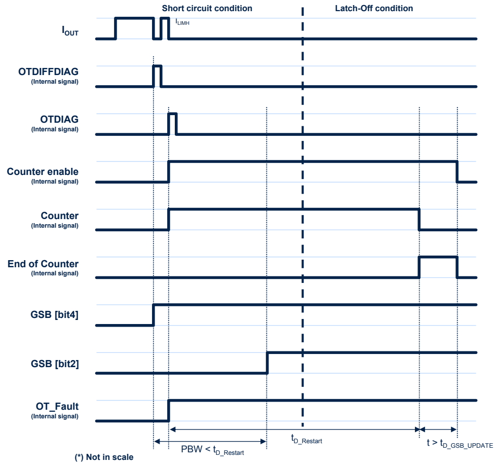
Figure 34. Normal mode - Short circuit – PBW < t_{D\_Restart}
