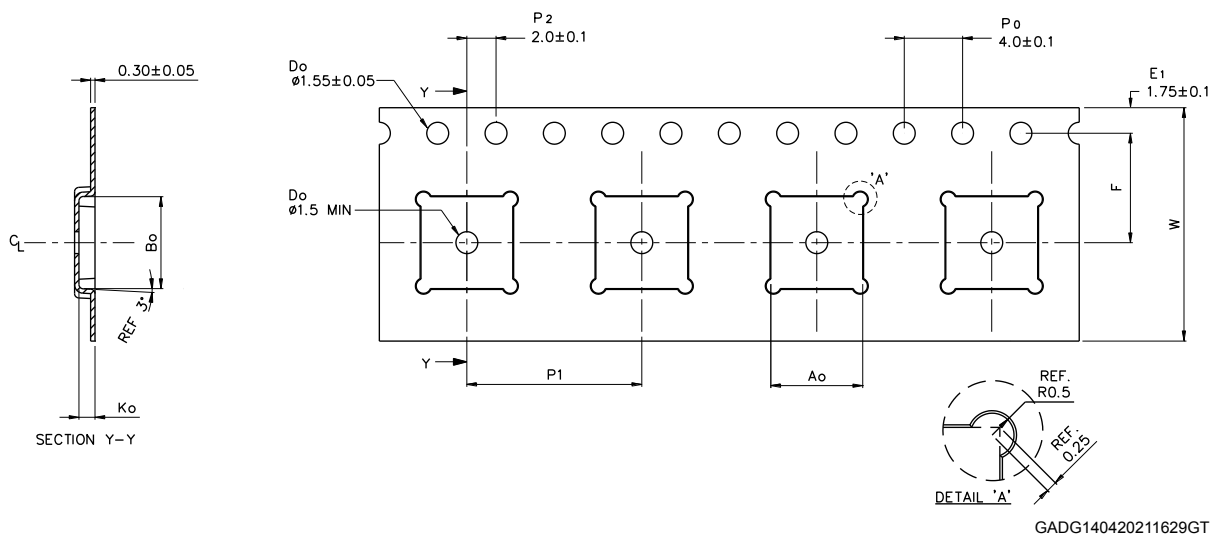
Figure 43. QFN 6x6 carrier tape
