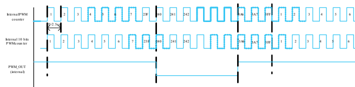
Figure 15. Resulting waveform 4
