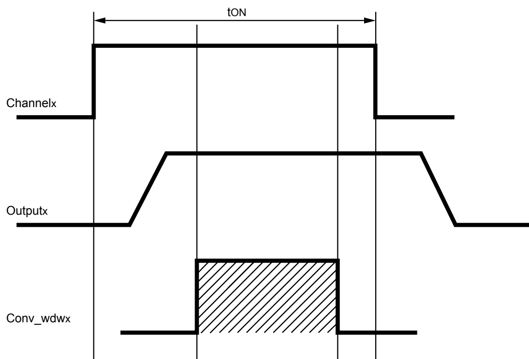
Figure 18. Conversion window generation
