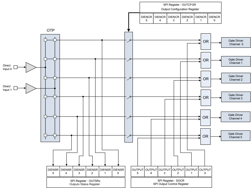
Figure 16. 56-channel direct input block diagram
