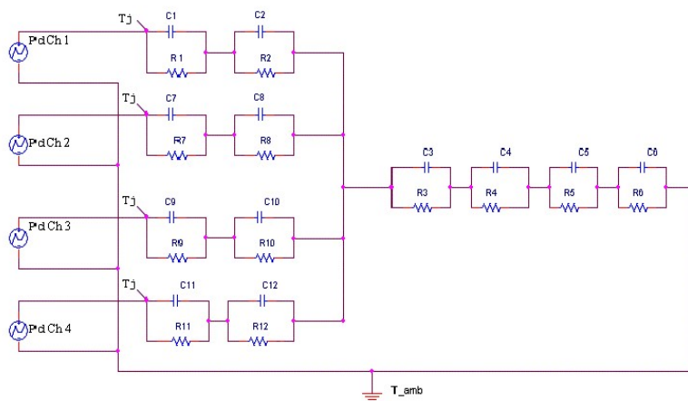
Figure 51. Thermal fitting model
