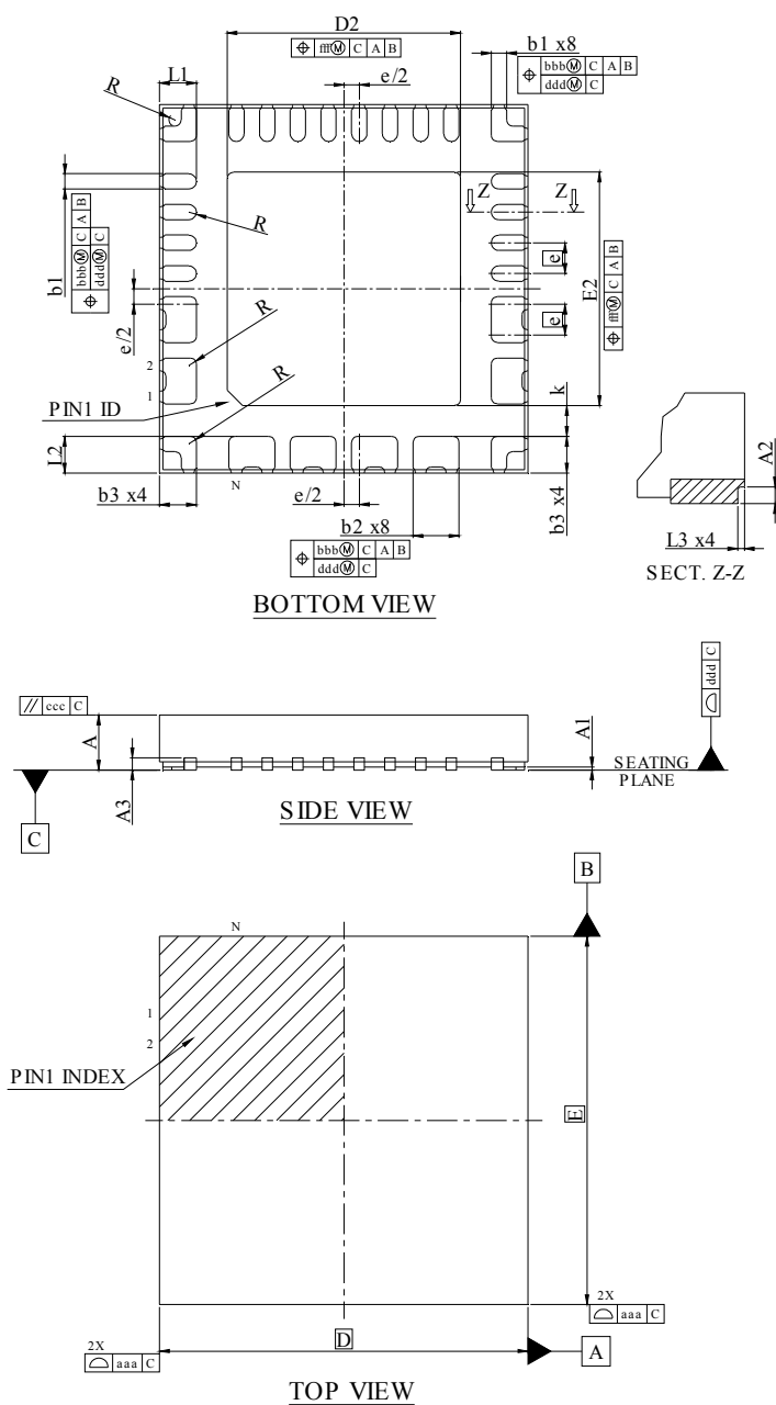
Figure 41. QFN 6x6 package outline
