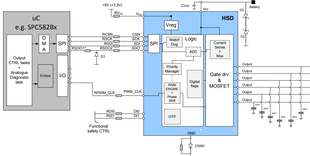
Figure 36. M0-9SPI application Schematic
