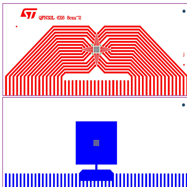
Figure 47. QFN 6x6 PCB 8 cm 2
