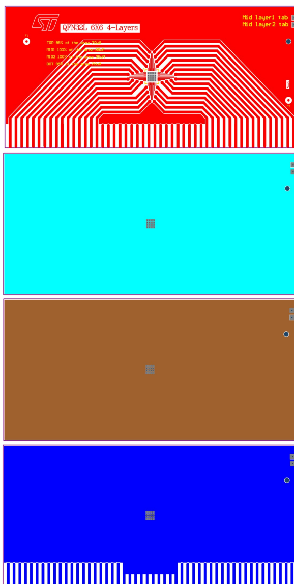
Figure 48. QFN 6x6 PCB 4 layers
