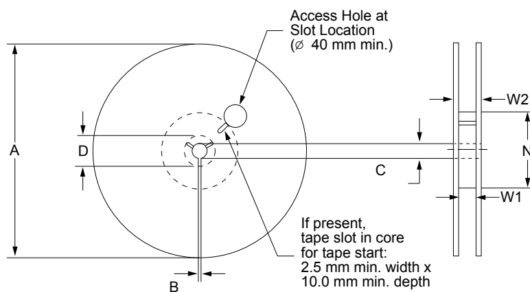
Figure 42. QFN 6x6 reel 13"
