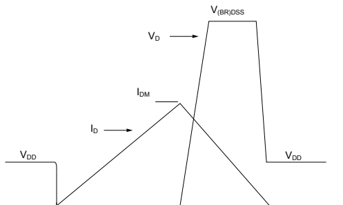
Figure 21. Unclamped inductive waveform
