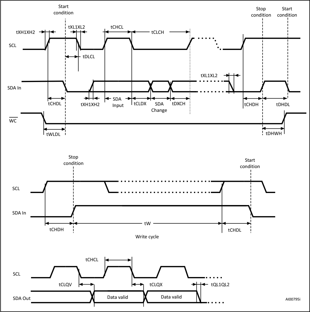
Figure 15. AC waveforms
