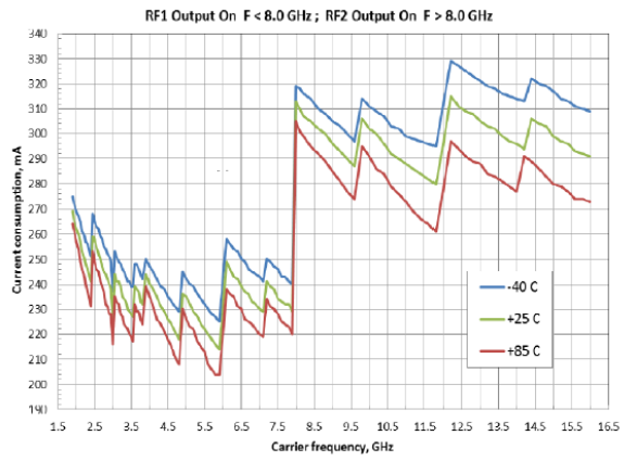
Figure 19. Overall current consumption vs. temperature (5.0 V supply, F_{\text{PFD}}=50 MHz)
