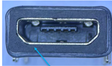
After: PA10T for housing
