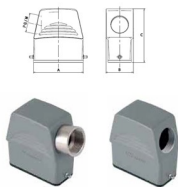
SIDE ENTRY HOOD
