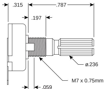
Dimensions (In.) (except where noted)
