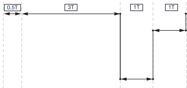
Fig. 21 - Timing Specification for Active Forced Mode
