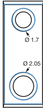
Fig. 9 - Light Hole Diameters
