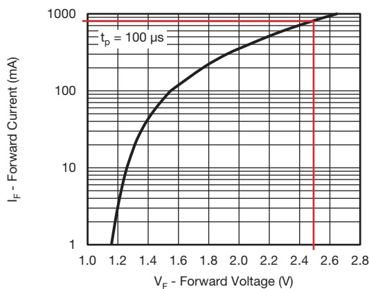
Fig. 12 - Forward Current vs. Forward Voltage
