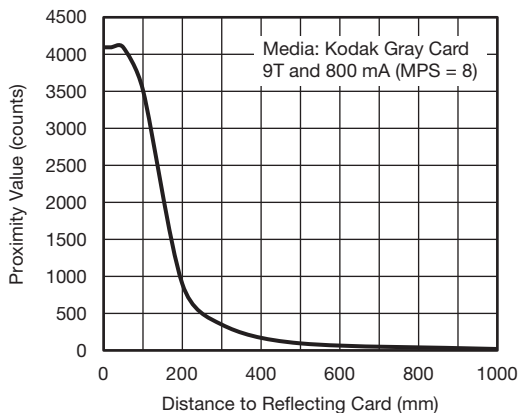
Fig. 17 - Proximity Value vs. Distance (axis with linear values)
