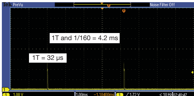
Fig. 19 - Proximity Measurements With PS_Duty = 1/160 and PS_IT = 1T
