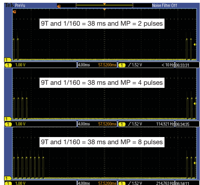
Fig. 13 - Proximity Measurements With PS_Duty = 1/160, PS_IT = 9T, and MP
