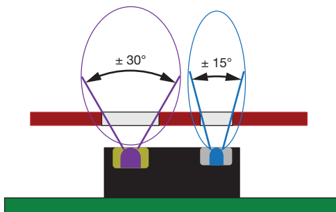
Fig. 7 - Emitter and Detector Angle
