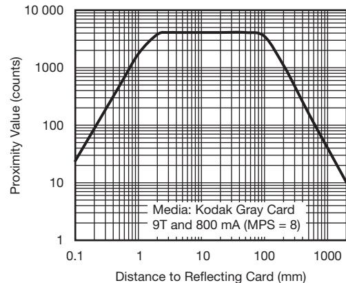
Fig. 16 - Proximity Value vs. Distance for PS_IT = 9T, MPS = 8 pulses and I IRED = 800 mA
