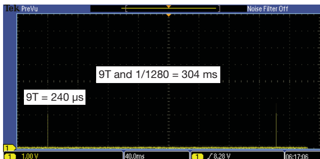
Fig. 20 - Proximity Measurements With PS_Duty = 1/1280 and PS_IT = 9T
