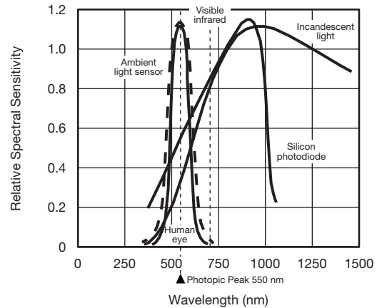
Fig. 22 - Relative Spectral Sensitivity vs. Wavelength
