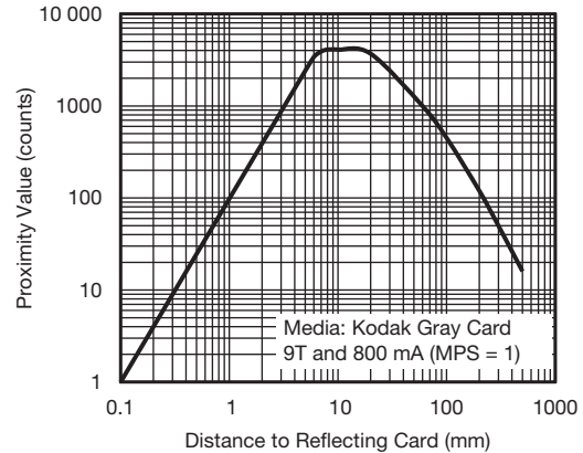
Fig. 15 - Proximity Value vs. Distance for PS_IT= 9T and I IRED = 800 mA
