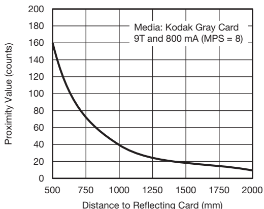
Fig. 18 - Proximity Counts vs. Distance Just for > 50 cm Distance
