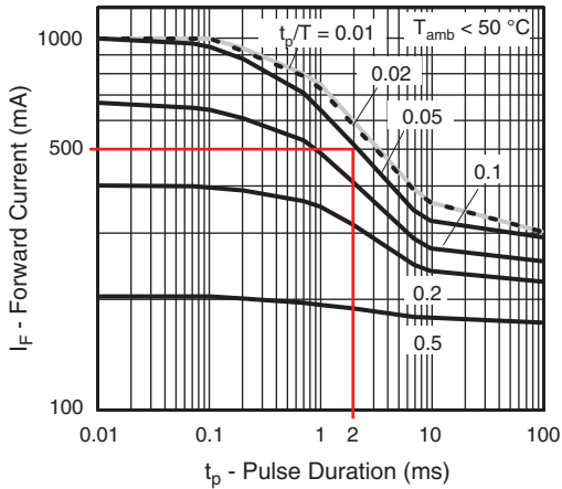
Fig. 14 - Pulse Forward Current vs. Pulse Duration
