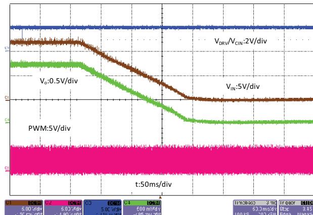
Power Off with V_{IN} Ramping Down V_{IN} = 12\text{ V} , V_{OUT} = 1.2\text{ V} , F_{SW} = 500\text{ kHz} , I_{OUT} = 1.2\text{ A}
