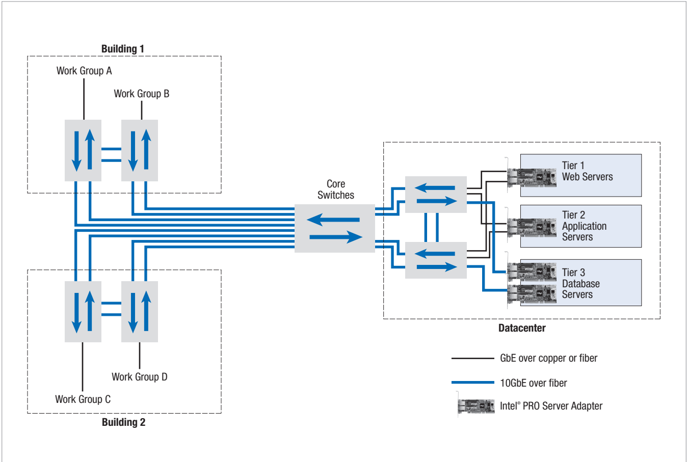
Figure 7. LAN with 10GbE backbone
