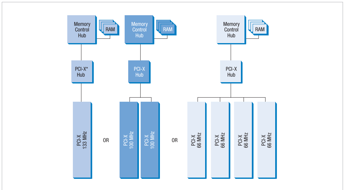
Figure 1. PCI-X* 1.0 specifies total slot capacity per bus speed
