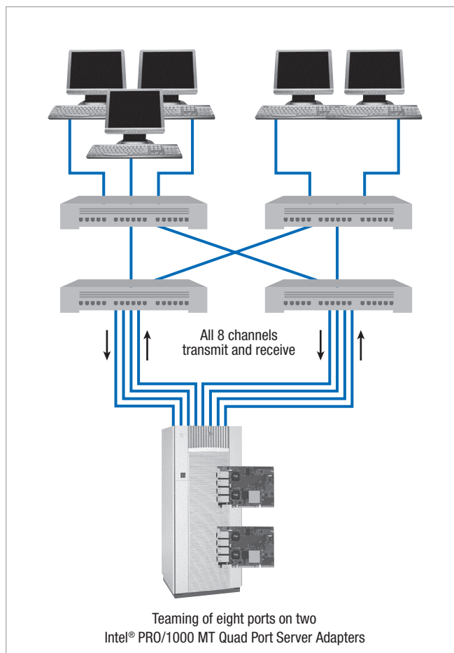
Figure 5. IEEE 802.3ad* link aggregation
