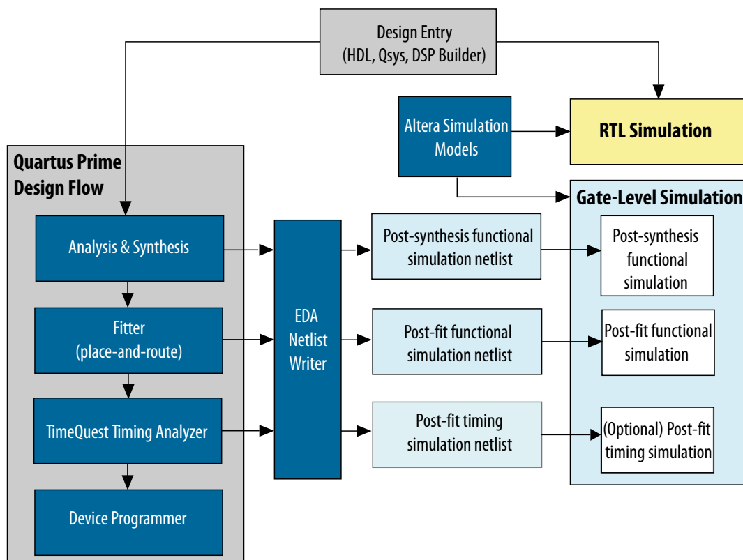
Figure 1-24: Simulation in Quartus Prime Design Flow
