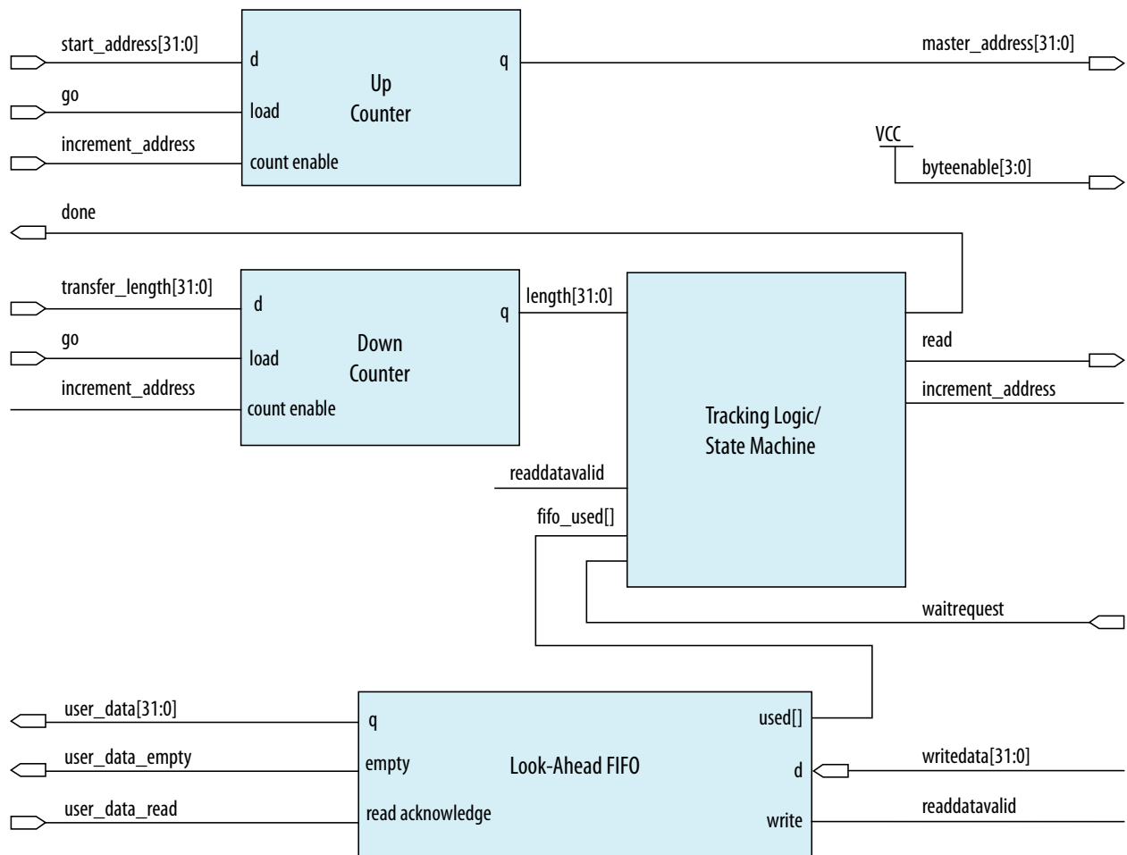
Figure 8-32: Pipelined Read Master
