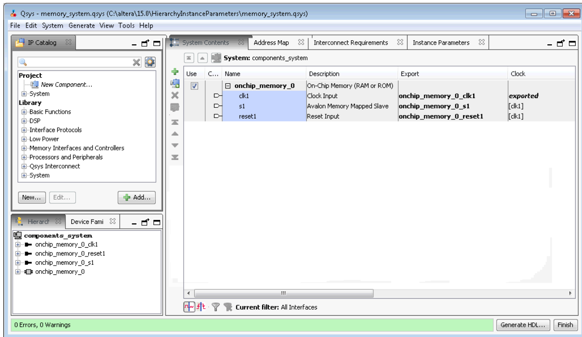
Figure 5-18: On-Chip Memory Component System and Instance Parameters (memory_system.qsys)
