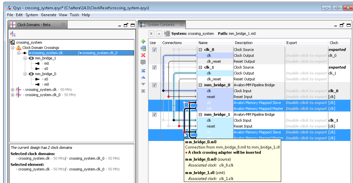
Figure 5-27: Clock Domain Crossings
