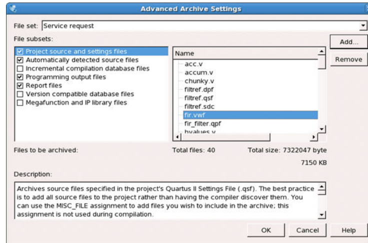
Figure 1-28: Archiving Project for Service Request
