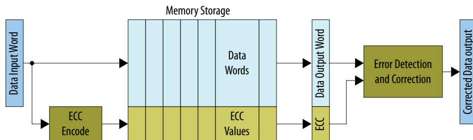
Figure 15-1: Memory Storage
