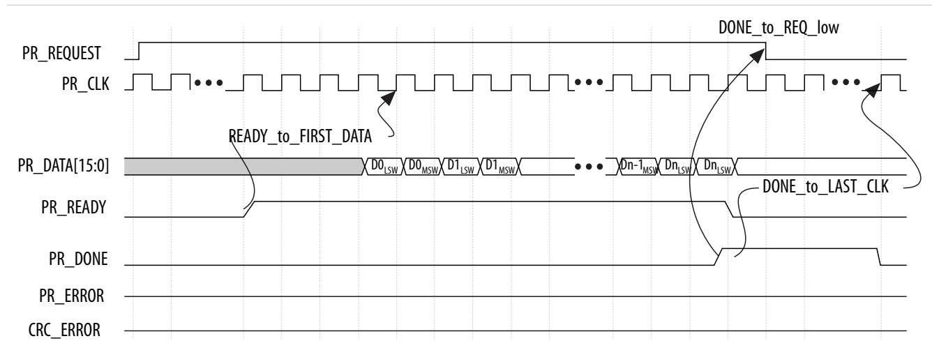
Figure 4-13: Partial Reconfiguration Timing Diagram
