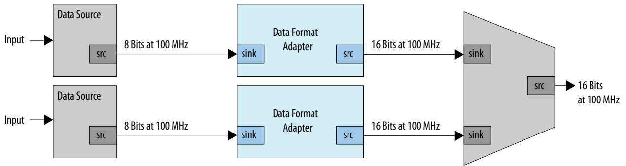
Figure 8-34: Data Path to Double Data Width and Maintain Original Frequency
