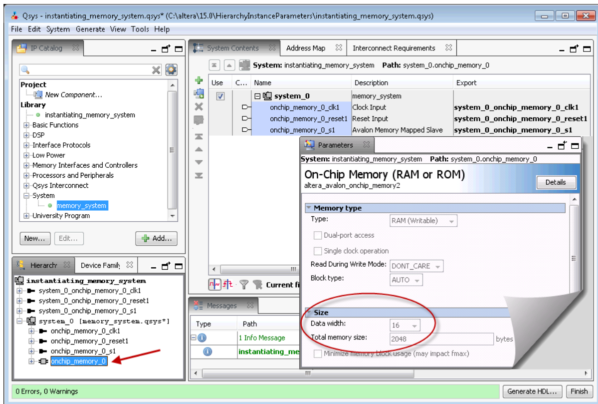
Figure 5-23: Changing the Values of Your Instance Parameters
