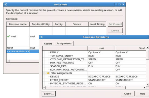
Figure 1-8: Comparing Project Revisions
