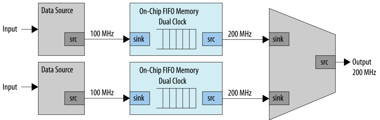
Figure 8-35: Data Path to Boost the Clock Frequency
