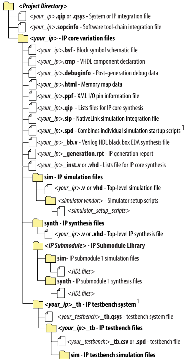
Figure 5-33: Files generated for IP cores and Qsys Systems
