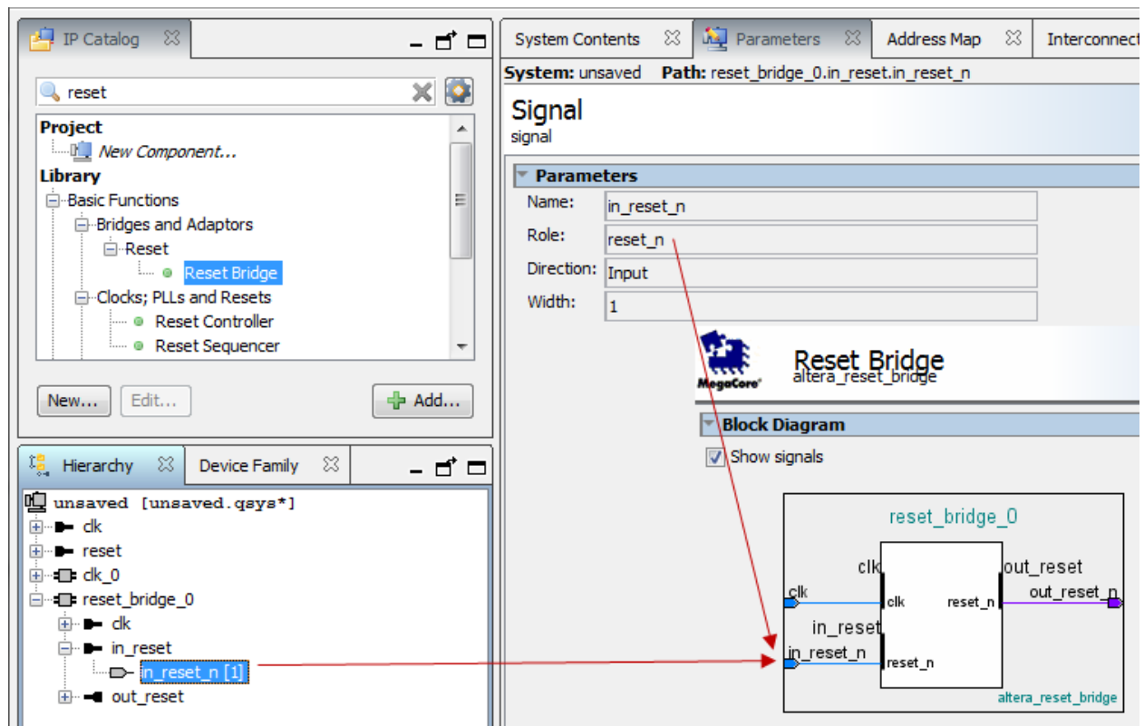
Figure 8-28: Reset Signal Active-Low
