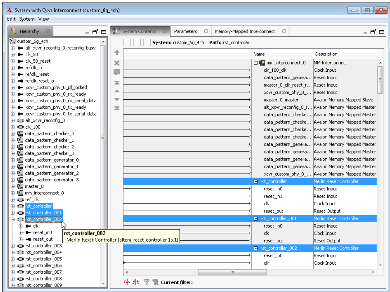
Figure 8-31: Qsys Interconnect
