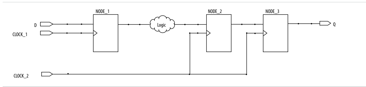
Figure 11-12: Undesired Condition 3
