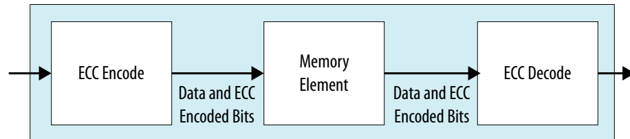
Figure 7-35: High-Level Implementation of RDATA FIFO with ECC Enabled
