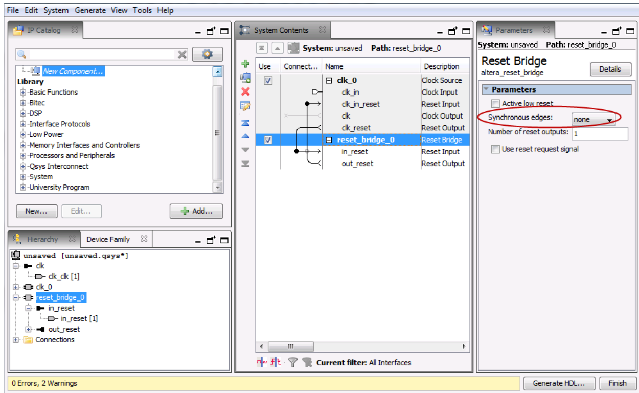
Figure 8-29: Synchronous Edges Parameter
