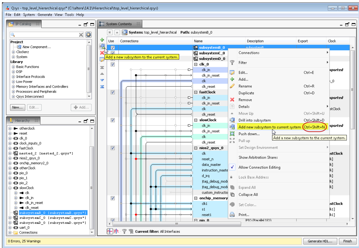
Figure 5-16: Add a Subsystem to Your Qsys Design
