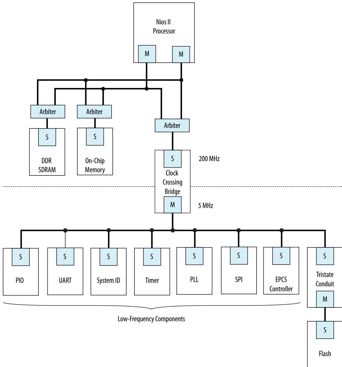
Figure 8-24: Reducing Power Utilization Using a Bridge to Separate Clock Domains
