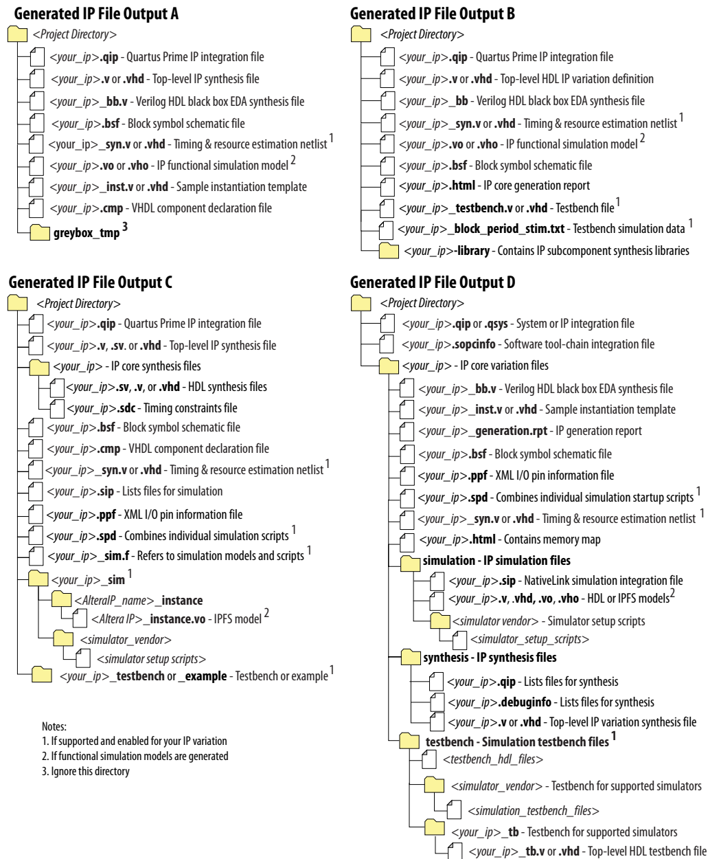
Figure 1-18: IP Core Generated Files (Legacy Parameter Editors)
