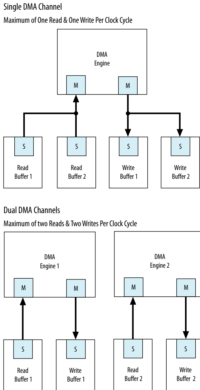
Figure 8-7: Single or Dual DMA Channels
