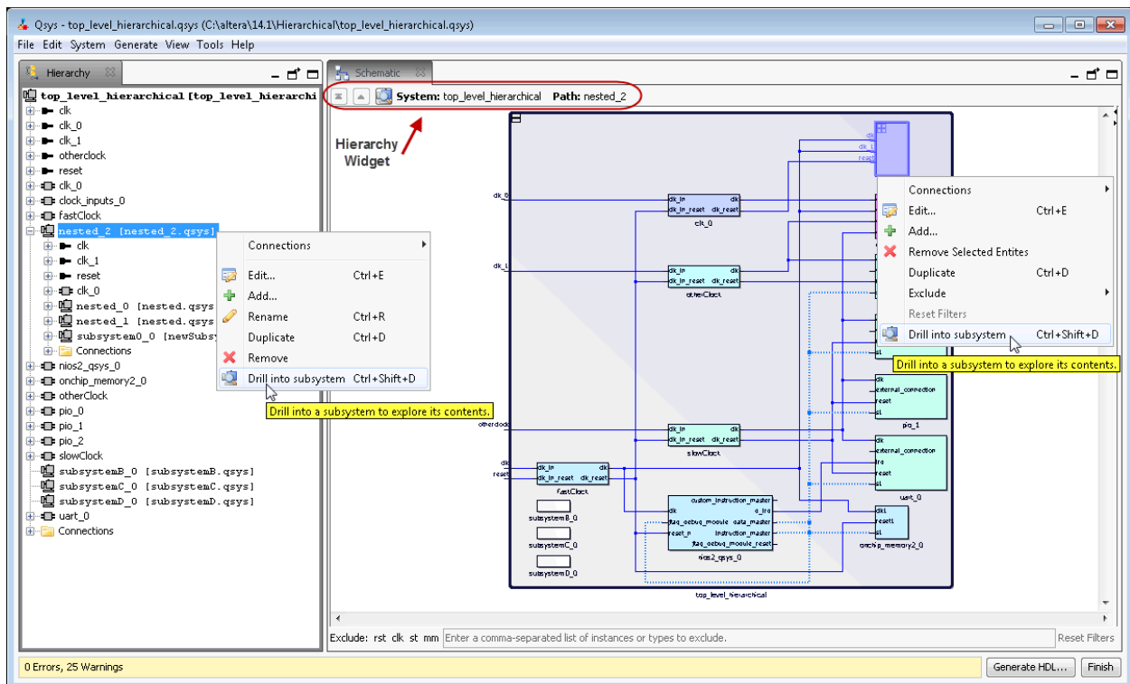
Figure 5-17: Drill into a Qsys System to Explore its Contents
