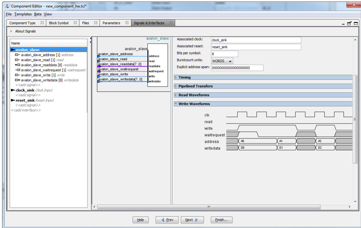
Figure 6-4: Qsys Signals &amp; Interfaces tab
