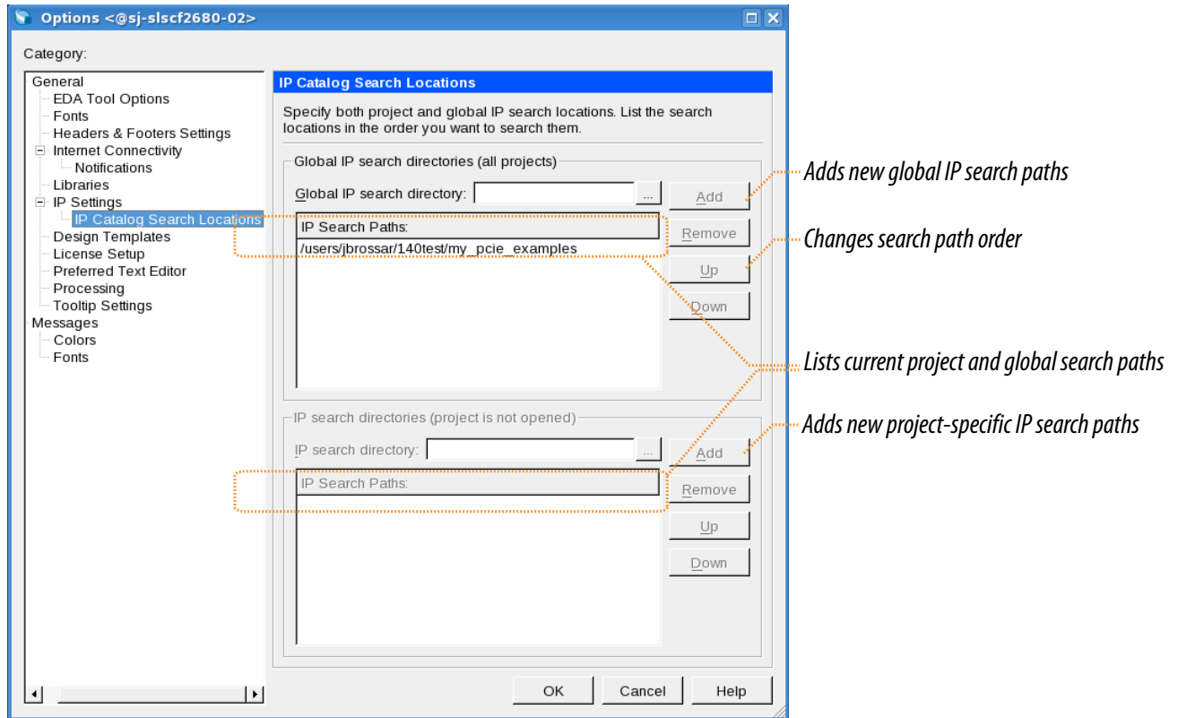
Figure 1-12: Specifying IP Search Locations
