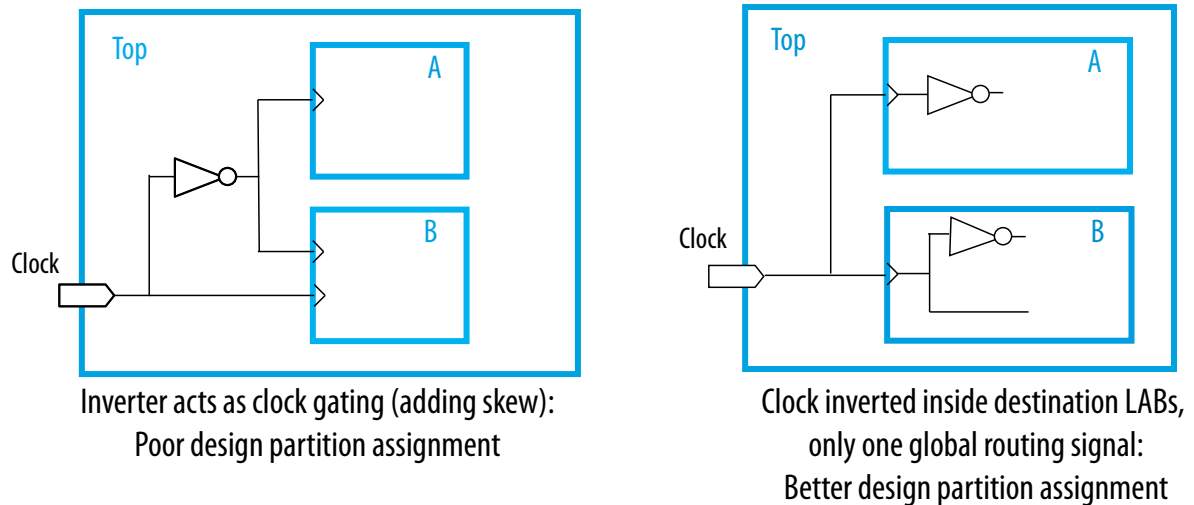
Figure 14-8: Inverting Clock Signal in Destination Partitions
