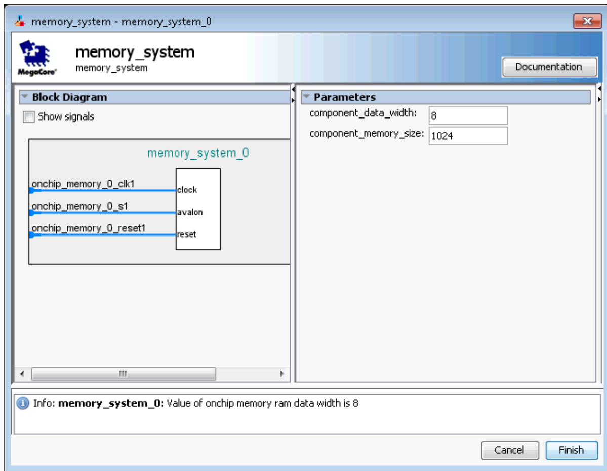
Figure 5-20: Preview Your Instance in the Parameter Editor
