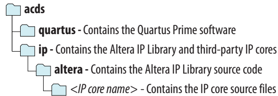
Figure 1-13: IP Core Installation Path
