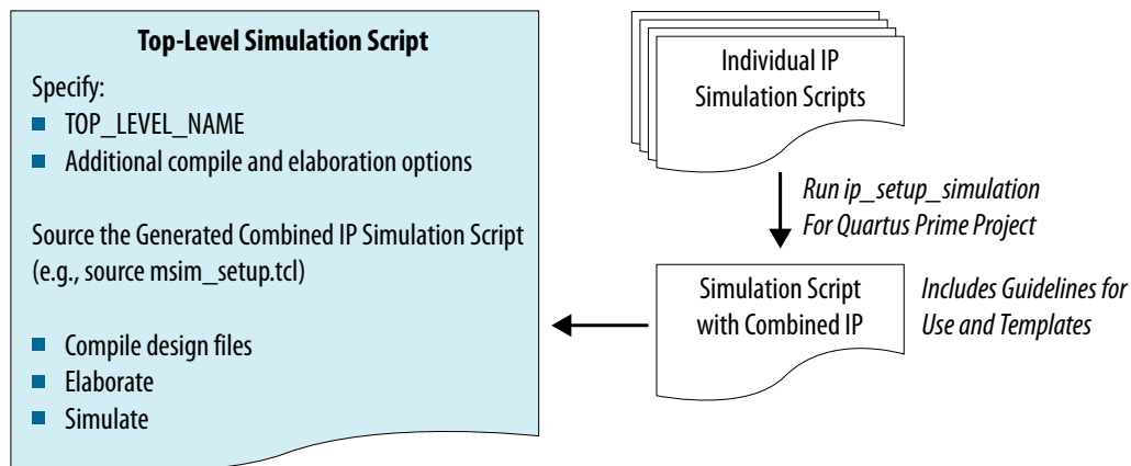
Figure 1-25: Incorporating IP Simulation Scripts into Top-Level Script
