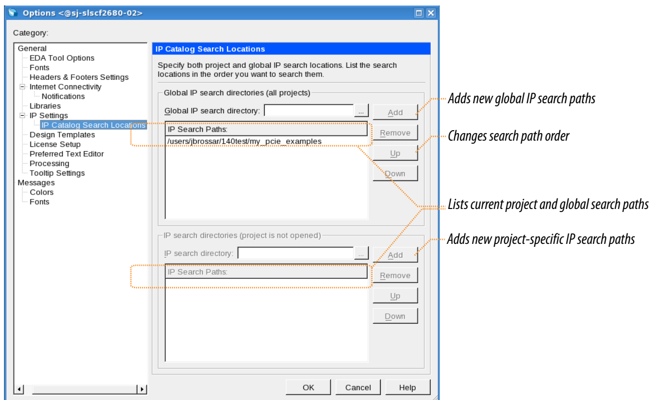
Figure 5-2: Specifying IP Search Locations
