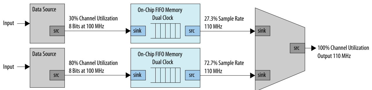
Figure 8-33: Data Path that Doubles the Clock Frequency
