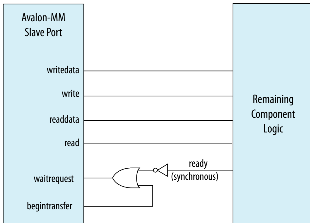
Figure 8-25: Variable Latency
