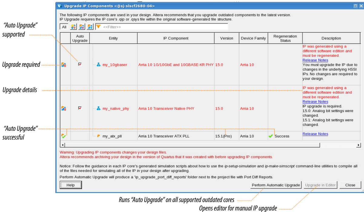
Figure 1-20: Upgrading IP Cores
