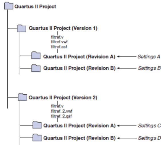
Figure 1-27: Quartus Prime Version-Compatible Database Structure
