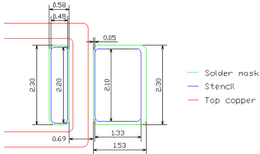
Figure 15: Recommended PCB solder pad layout for LUXEON 3030 2D.
