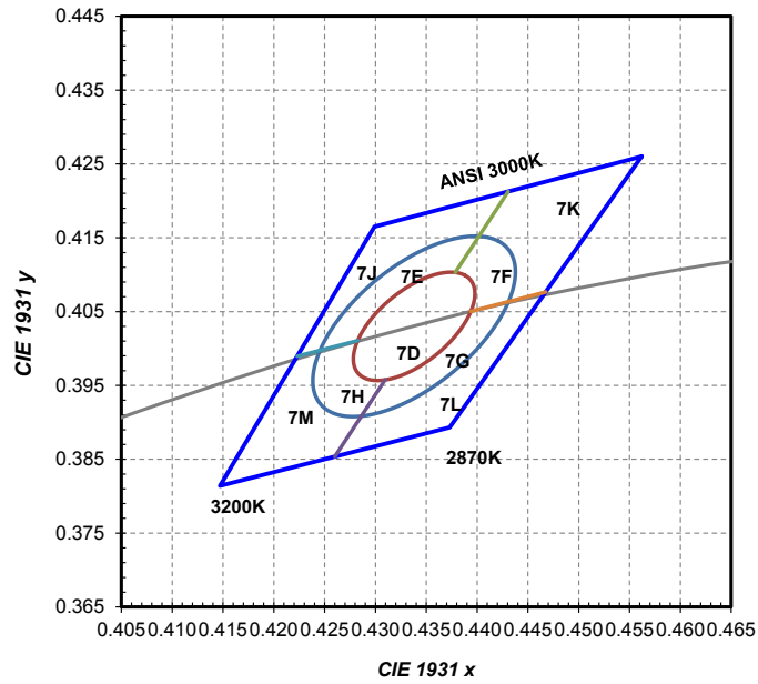
Figure 7: Color bin structure for LUXEON 3030 2D 3000K.
