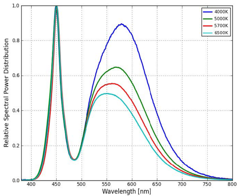
Figure 1a: Typical normalized power vs. wavelength for L130-xx80003000W21 120mA, Tj=25°C.
