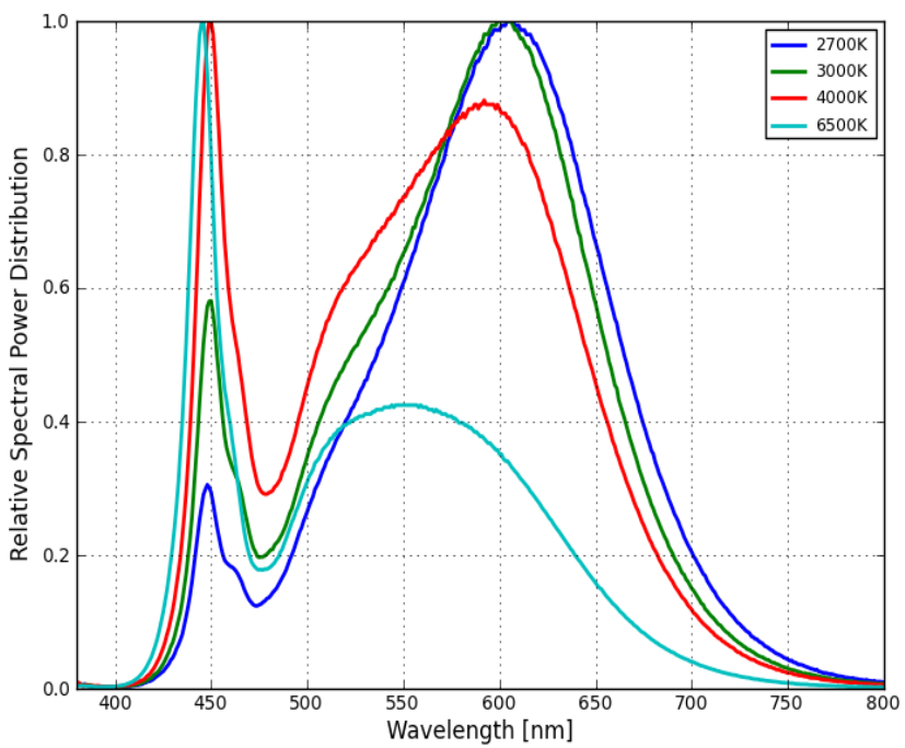
Figure 1b: Typical normalized power vs. wavelength for L130-xx70003000W21 at 120mA, Tj=25°C.
