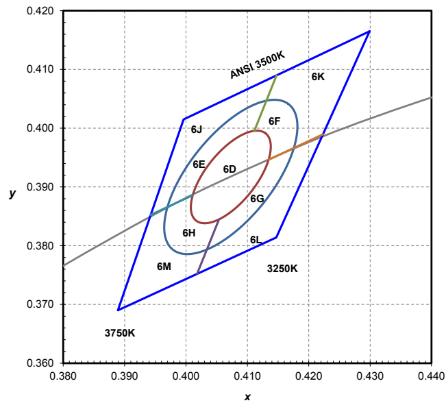
Figure 8: Color bin structure for LUXEON 3030 2D 3500K.
