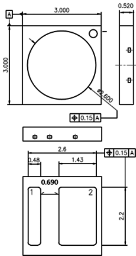
Figure 13: Mechanical dimensions for LUXEON 3020 2D.
