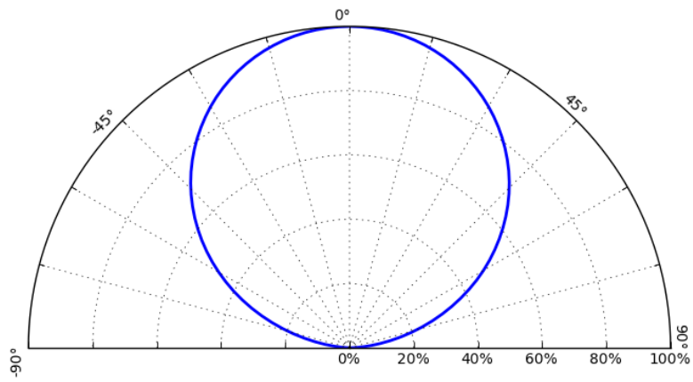
Figure 4b: Typical polar radiation pattern for L130-xxxx003000W21 at 120mA, T j =25°C.
