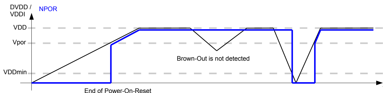
Figure 5.4.2.1-1 Power-On-Reset timing diagram
