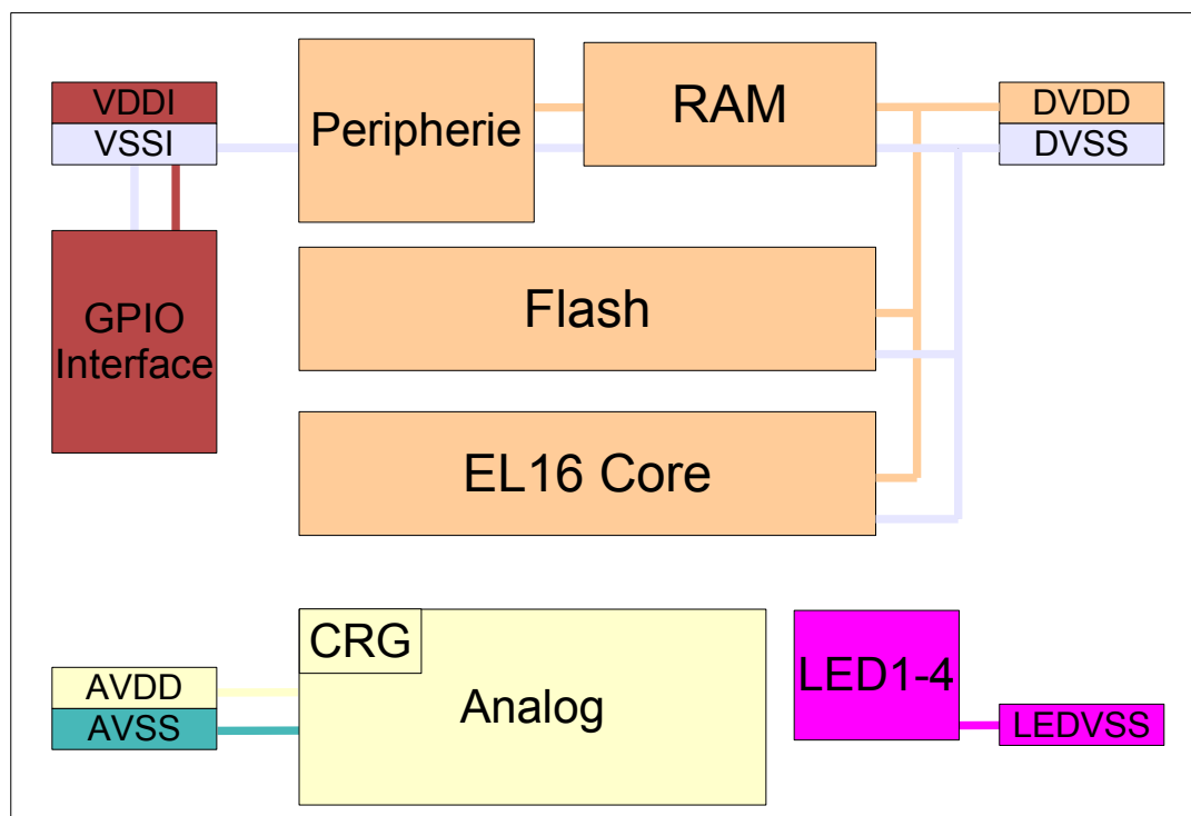
Figure 5.2.1-1 Block Diagram of Power Supply
