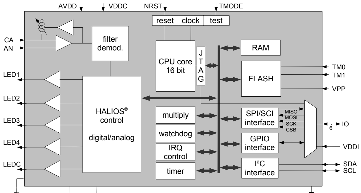
Figure 2-1 Block Diagram
