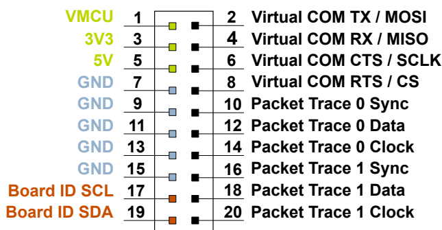
Figure 4.5 Simplicity Connector
