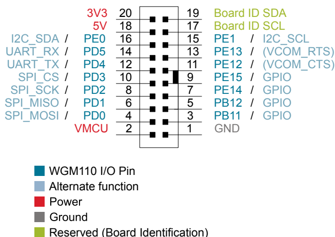
Figure 4.3 Expansion Header
