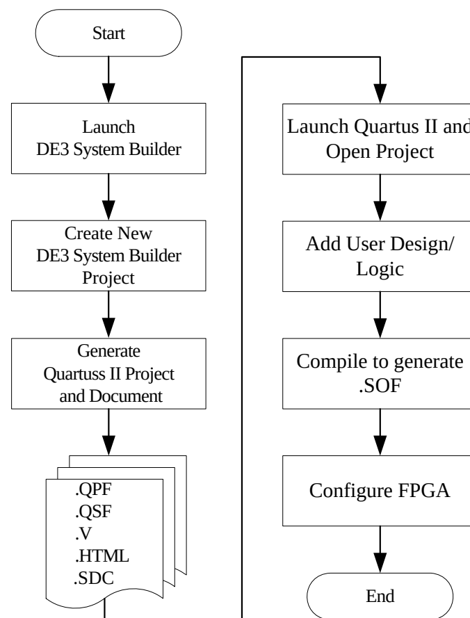
Figure 4.1. The general design flow of building a design for the DE3 board via the DE3 System Builder
