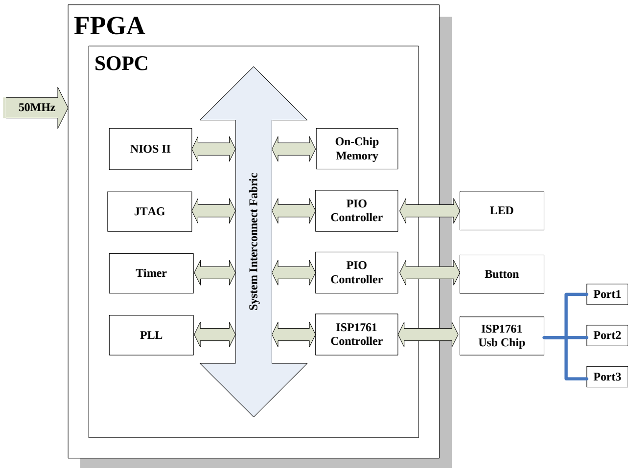
Figure 5.2. Hardware Block Diagram of the USB-Host Demonstration
