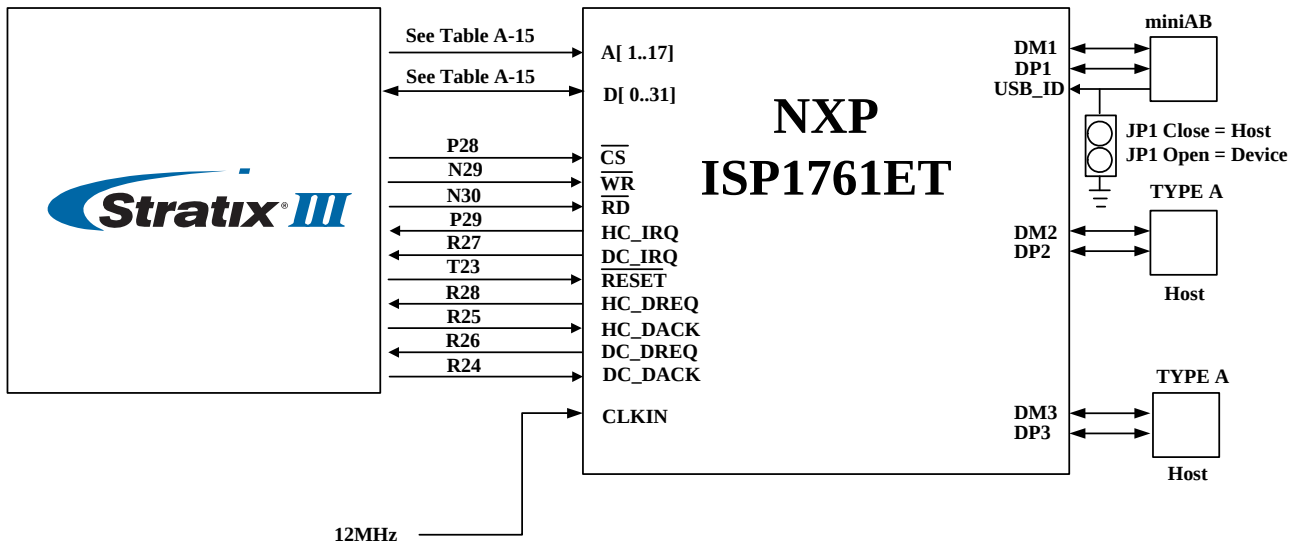
Figure 2.17. Connections between the USB OTG and Stratix III device
