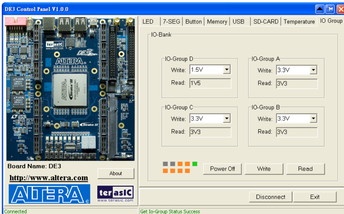
Figure 3.15. Reading the V_{CCIO} level of all I/O Groups
