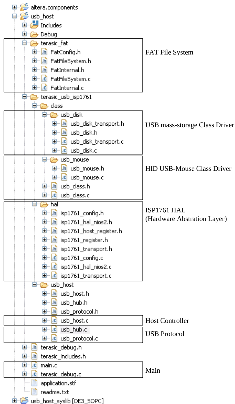
Figure 5.5. Source Code List of the USB-Host Demonstration
