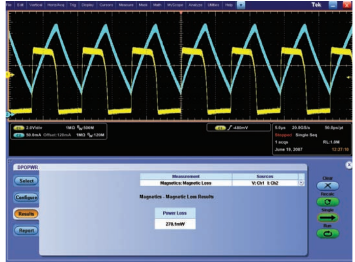
Figure 16. Power loss at single-winding inductor as measured by DPOWRL.
