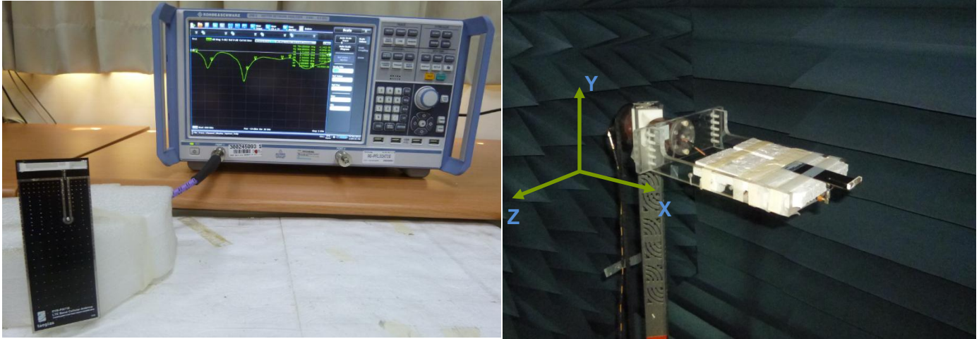
Figure 1. Impedance measurements (left hand) and peak gain, average gain, efficiency and radiation pattern measurements (right hand)
