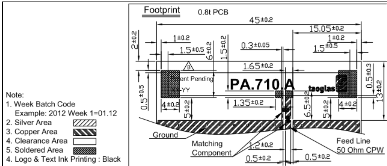
Figure 15. Layout dimensions of the Warrior PA710 Antenna.
