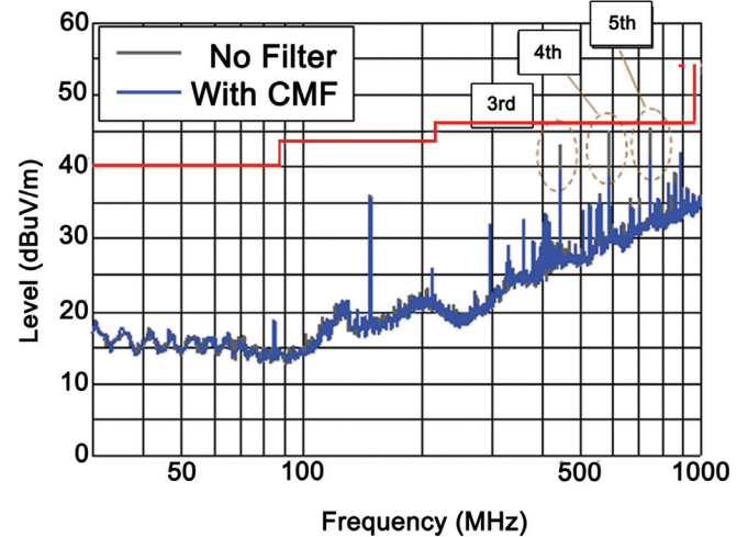
Fig 13: EMI Scan using 1080p resolution (the contribution of the common mode filter is more visible in reducing the high frequency harmonics)
