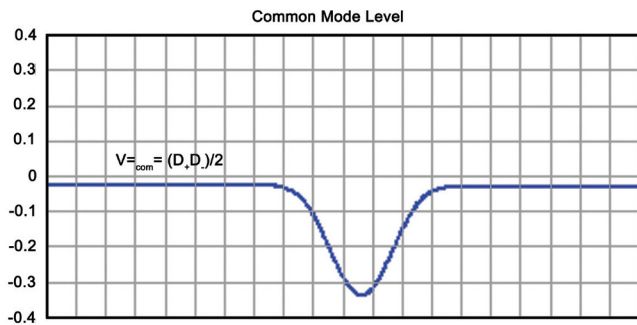
Figure 19: a) Skew measurement and b) Common mode voltage
