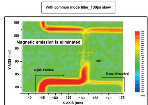
Figure 22: Magnetic scan with skewed input signal and using filter
