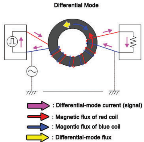
Figure 5 : Differential mode signal and noise cancel mechanism
