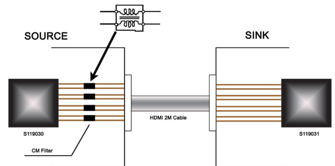
Figure 11: Common mode filter connection drawing
