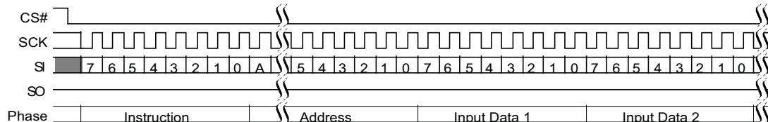
Figure 10.51 Page Program (PP 02h or 4PP 12h) Command Sequence
