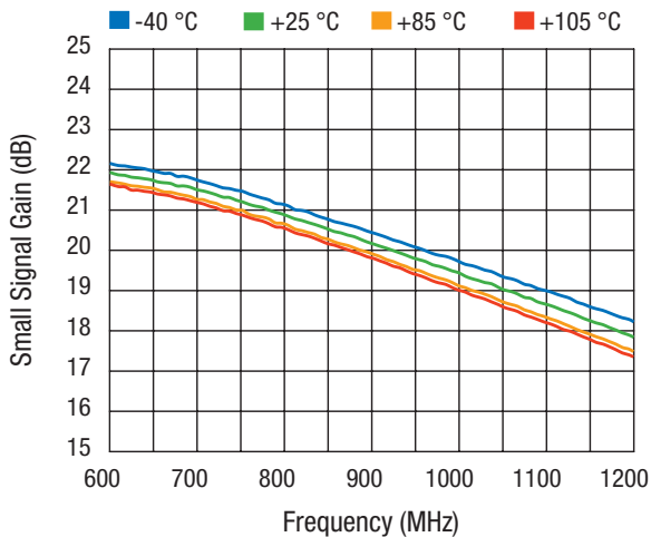
Figure 5. Small Signal Gain
