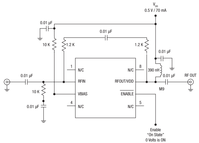
Figure 12. Low Frequency Schematic With Feedback
