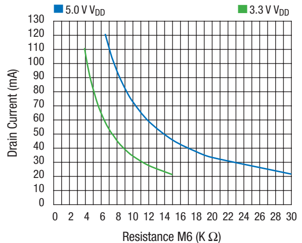
Figure 2. Bias Currents vs. External Resistance
