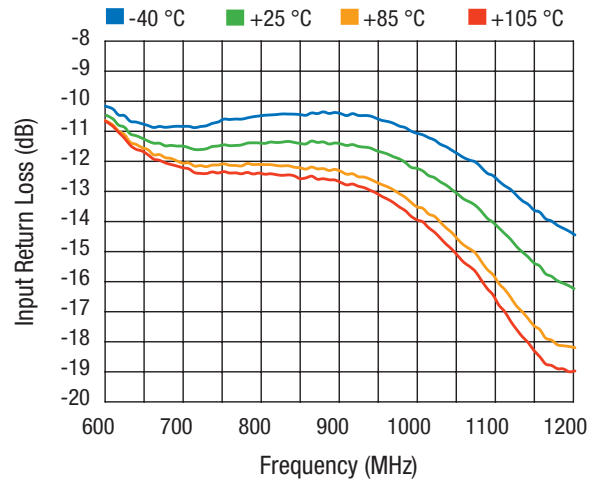
Figure 6. Input Return Loss
