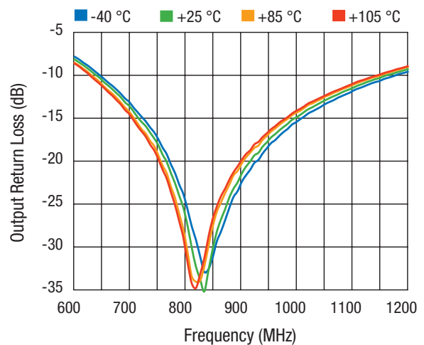
Figure 8: Output Return Loss
