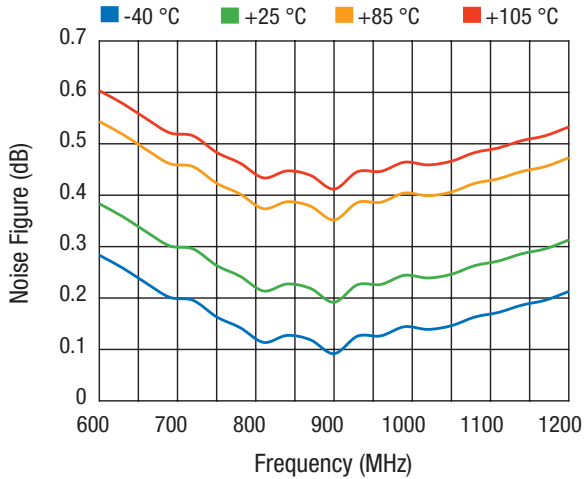
Figure 9. Noise Figure
