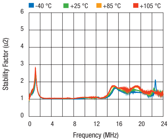
Figure 11. Stability Factor (u2)
