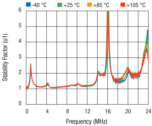
Figure 10. Stability Factor (u1)
