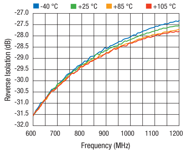
Figure 7. Reverse Isolation
