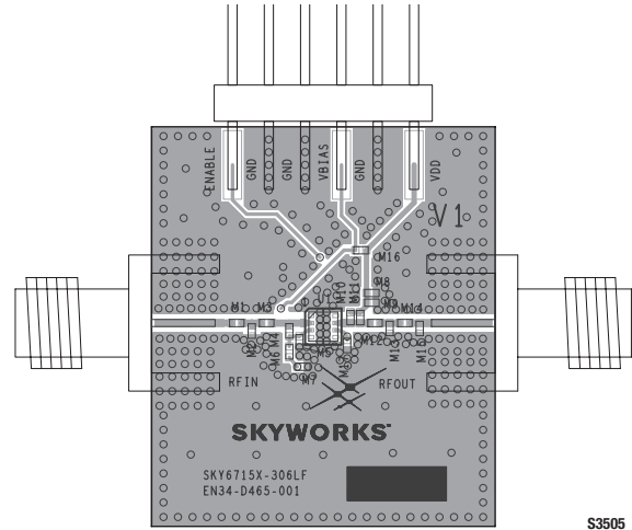
Figure 3. Applications Circuit
