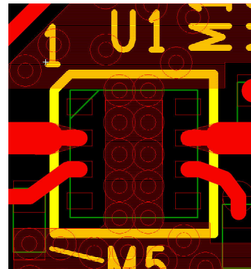
Figure 4. Ground Via Land Pattern
