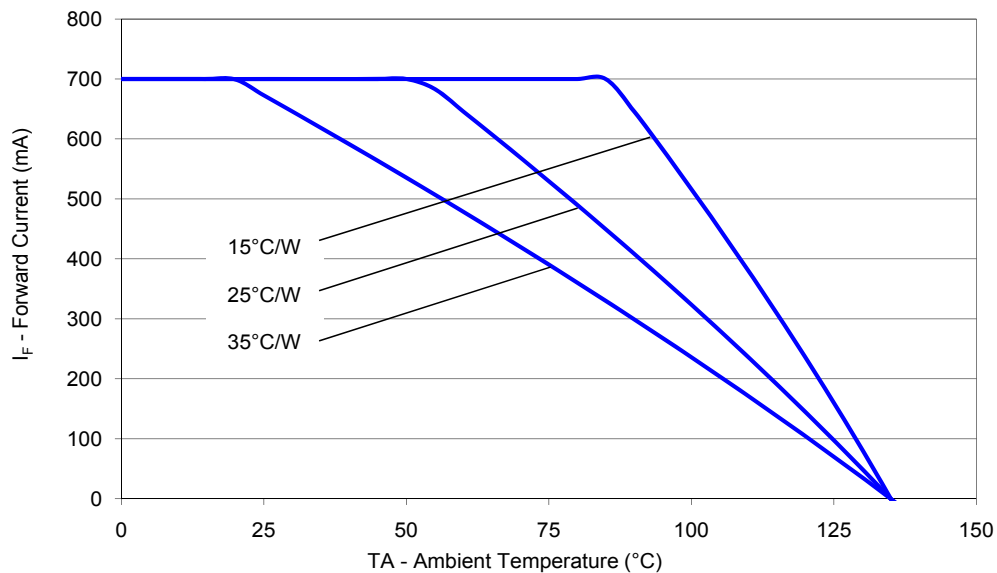
Figure 15. Maximum forward current vs. ambient temperature, based on T_{JMAX} = 135^{\circ}\text{C} .
