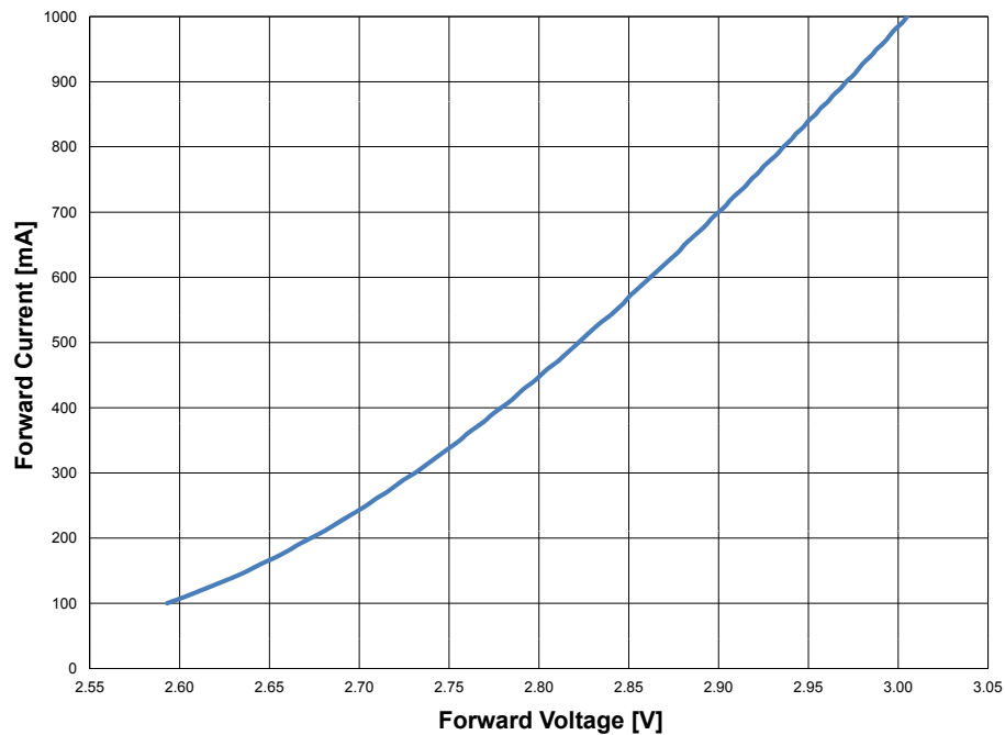
Figure 13. Forward current vs. forward voltage.
