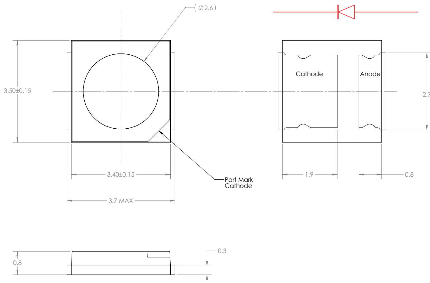
Figure 1. Package outline drawing.
