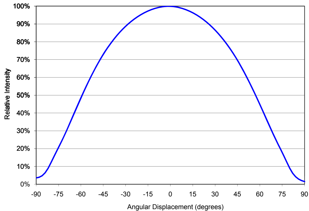
Figure 10. Cartesian plot of typical luminous intensity.
