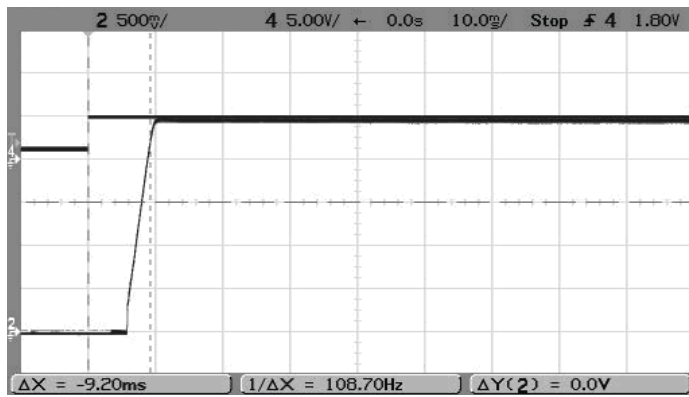
On/Off Enable Delay (Vin=13.8V, Vout=2.5V, Iout=6A, Cloud=0) Trace 4=Enable, Trace 2=Vout
