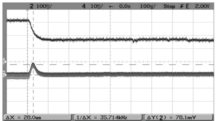
Step Load Transient Response (Vin=12V, Vout=2.5V, Cloud=0, Iout=6A to 3A) Trace 2=Vout, 100 mV/div. Trace 4=Iout, 2A/div.
