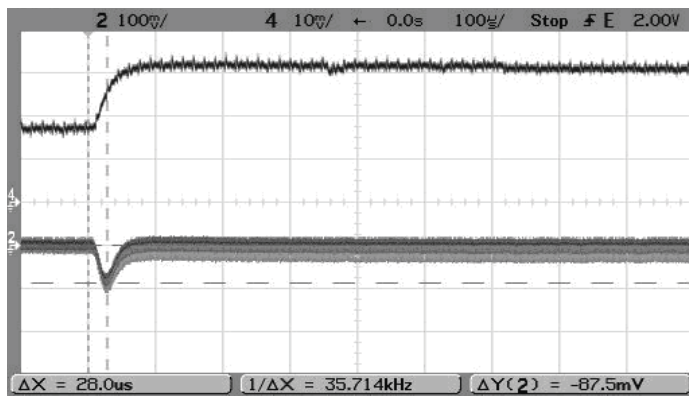
Step Load Transient Response (Vin=12V, Vout=2.5V, Cloud=0, Iout=3A to 6A) Trace 2=Vout, 100 mV/div. Trace 4=Iout, 2A/div.
