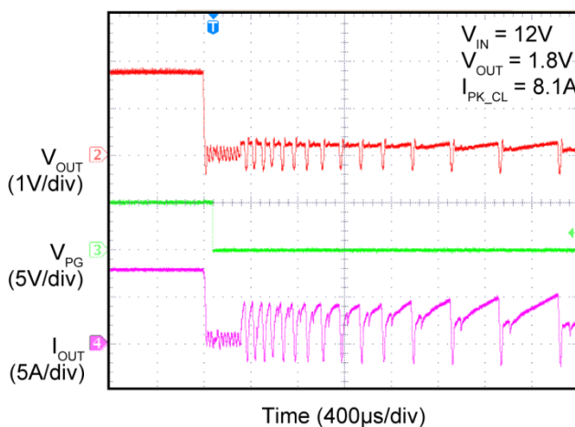
Peak Current Limit Threshold
