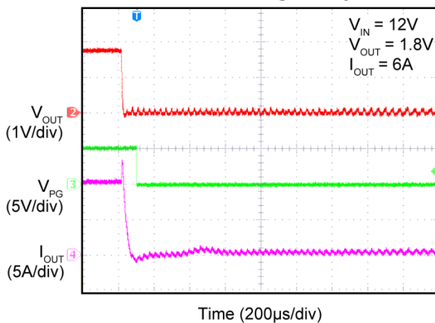
Short Circuit During Steady State
