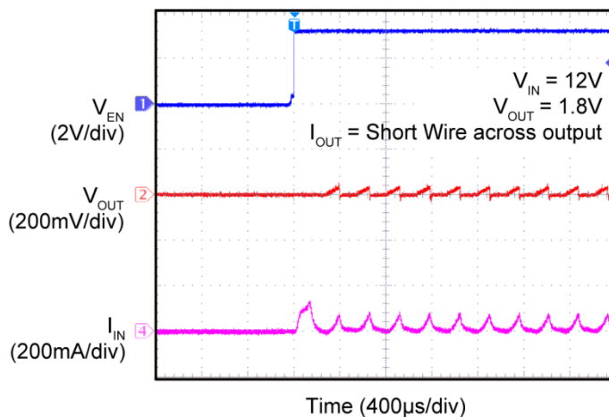
Enabled Into Short
