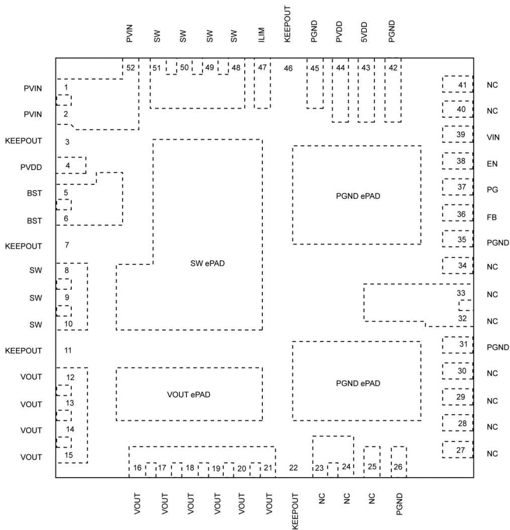
52-Pin 8mm × 8mm × 3mm QFN (Top View)
