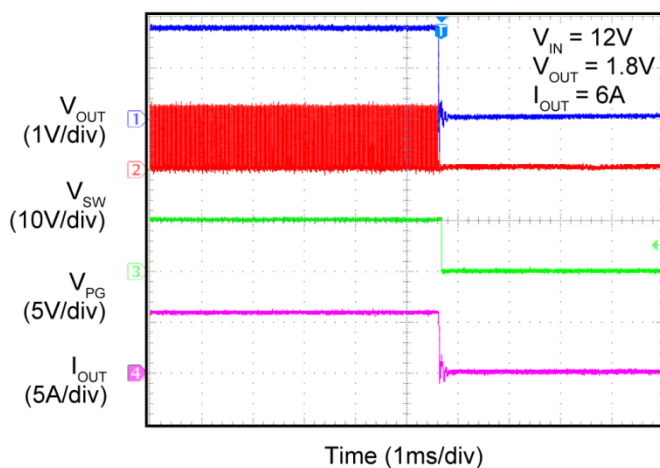
Thermal Shutdown
