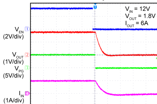
Enable Turn-On Delay and Fall Time
