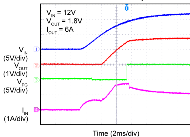
Inrush with 3000μF
