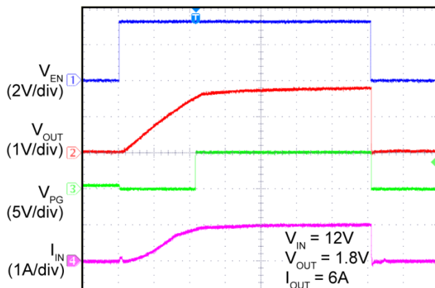
Enable Turn-On/Turn-Off
