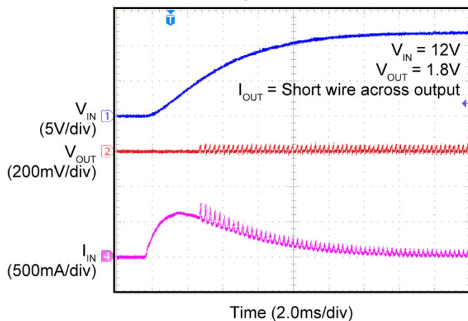
Power Up into Short Circuit
