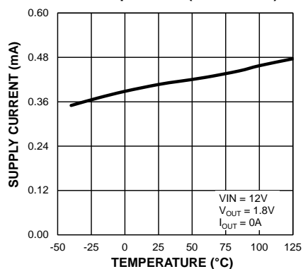
VIN Operating Supply Current vs. Temperature (MIC45116-1)
