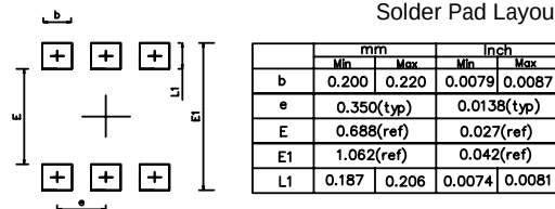
SOT 963 Solder Pad Layout
