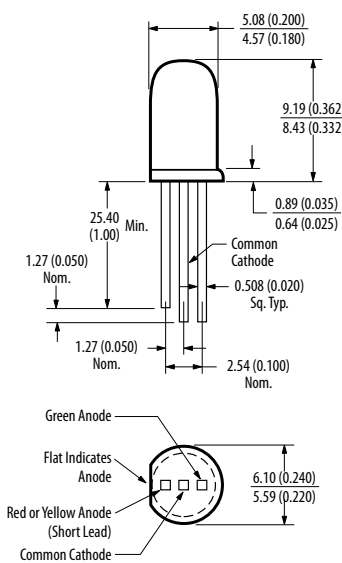
5 mm (T1-3/4) LED Lamps - Bicolor
