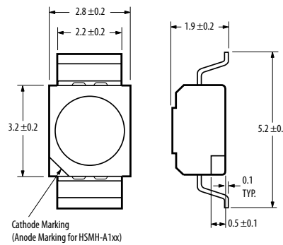
PLCC-2 Reverse Mount
