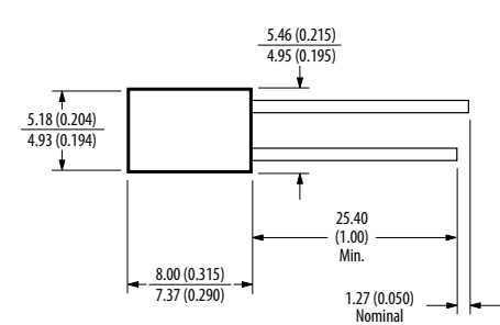
2 x 5 mm Rectangular LED Lamps Package
