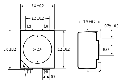
Super 0.5W Power PLCC-4
