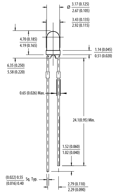
3 mm (T1) LED Lamps Package
