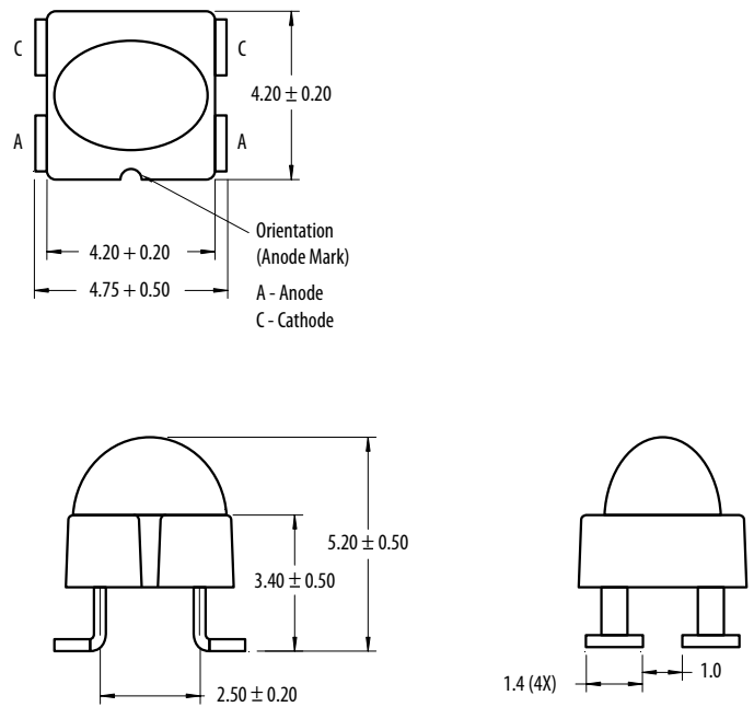
Package Drawing B
