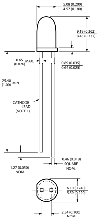
5 mm (T1 3/4) LED Lamps Package
