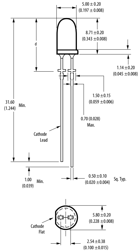
B: Standoff
