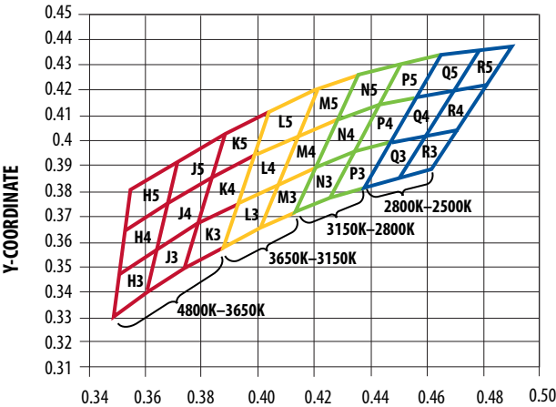
Color Coordinates Chart for ASMT-QYBx
