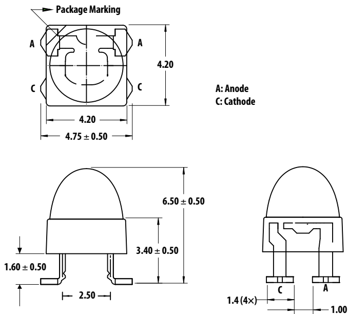
Package Drawing C
