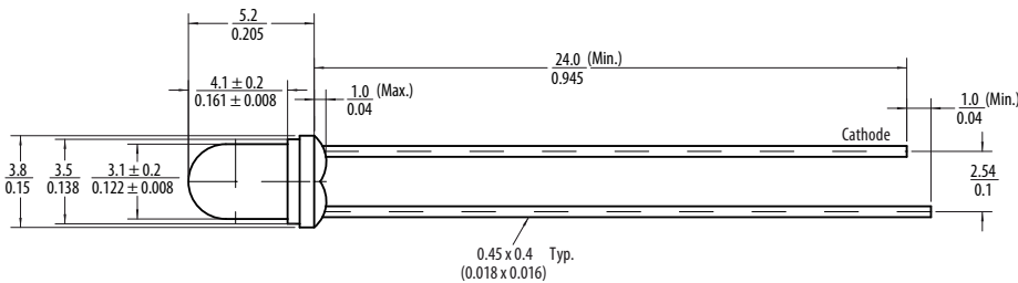
3 mm (T1) AlInGaP LED Lamps Package
