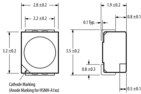
PLCC-2 Top Mount
