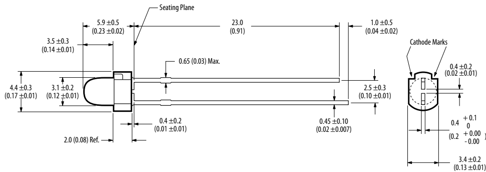
3 mm (T1) AlInGaP LED Lamps Package
