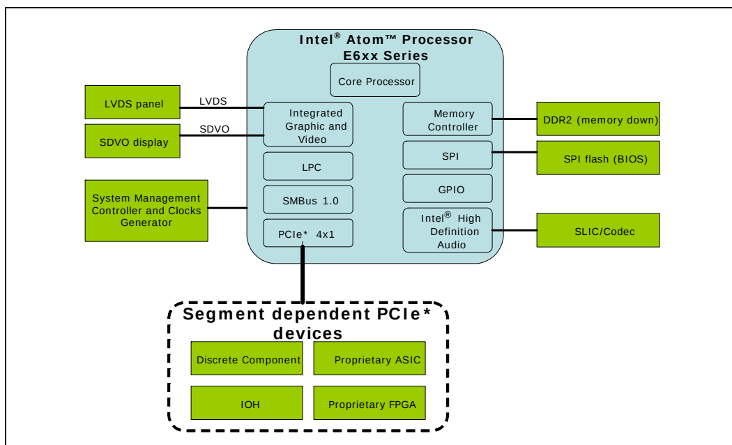
Figure 1. System Block Diagram Example
