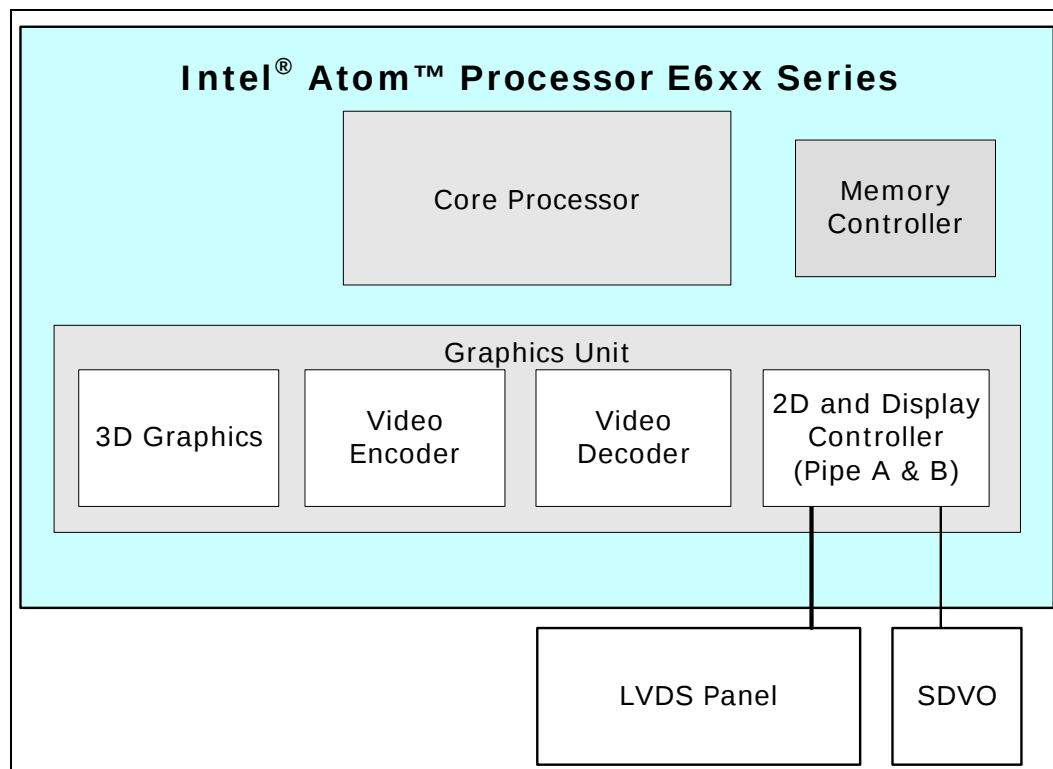
Figure 5. Graphics Unit
