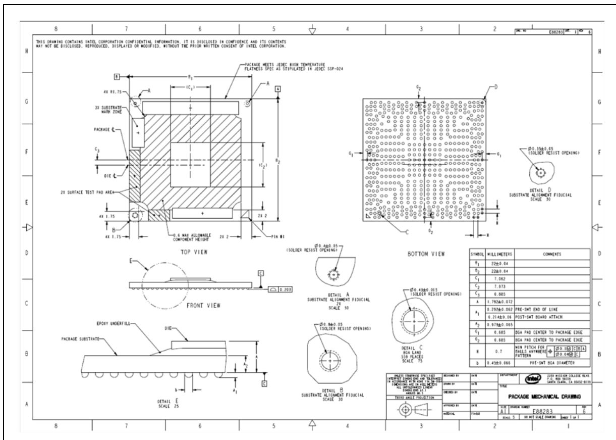
Figure 5-11. Mechanical Drawings
