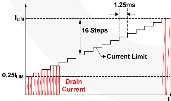
Figure 21. Internal Soft-Start
