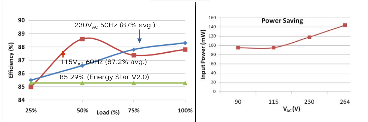
Figure 28. Measured Efficiency and Power Saving
