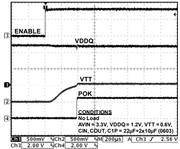
Startup with POK at 2A
