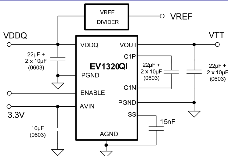
Figure 1. Simplified Applications Circuit
