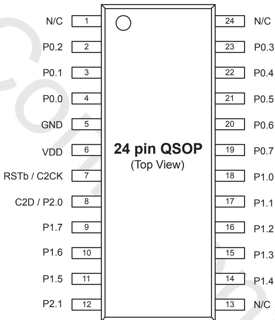
Figure 4.1. EFM8BB1x-QSOP24 Pinout
