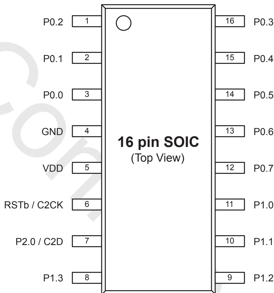
Figure 4.3. EFM8BB1x-SOIC16 Pinout
