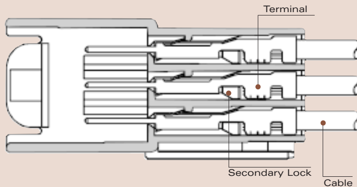
Male Connector
