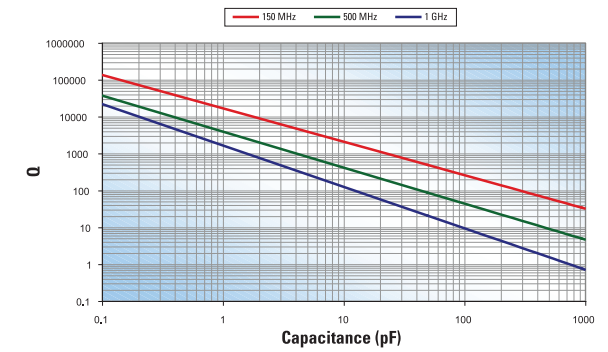
Q vs Capacitance DLI C18 CF Series
