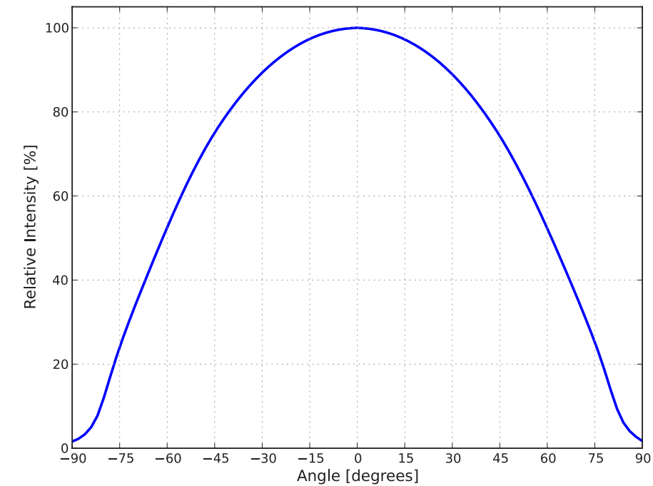
Figure 2: Typical radiation pattern for LUXEON M at 700mA, T j =85°C.
