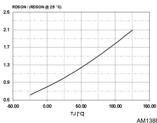
Figure 11. Main FET R_{DS(on)} vs. T_J
