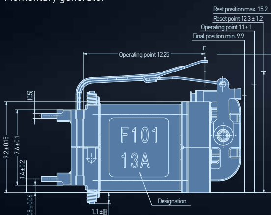
Momentary generator
