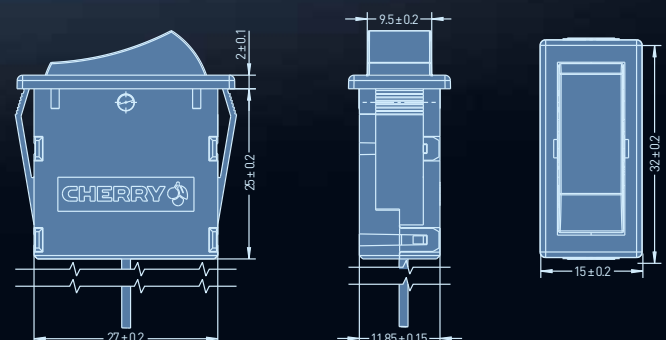
Rocker switch
