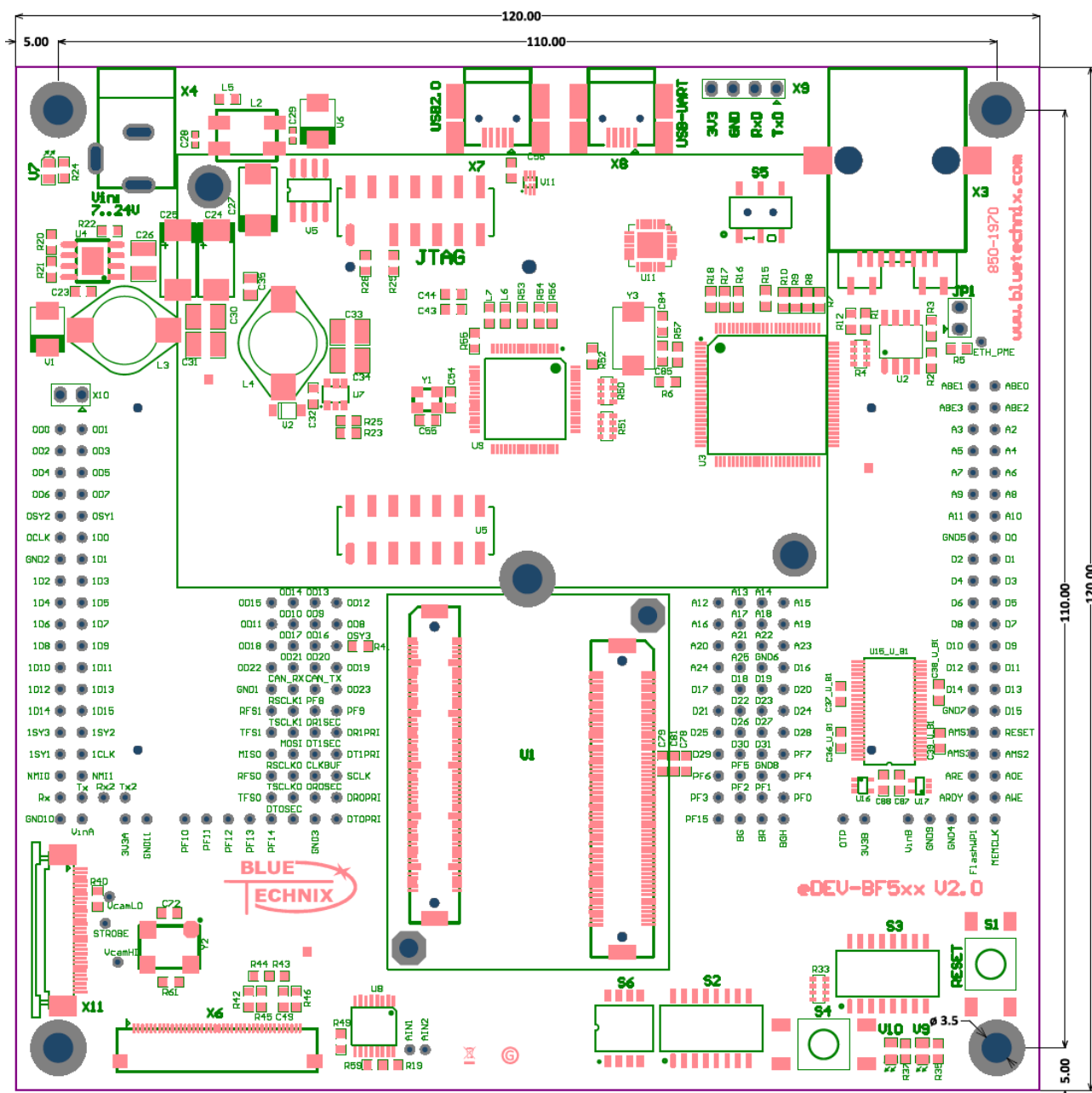
Figure 2-3: Mechanical outline top view
