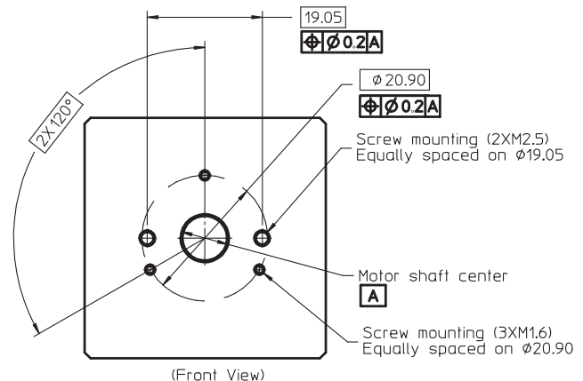
Figure 3. Recommended motor mounting dimension
