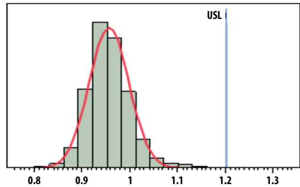
Figure 2. NF @ 2.4 GHz, V_{dd} 3\text{ V} ; V_{bias} 1.8\text{ V} Nominal = 0.95 dB, USL = 1.2 dB
