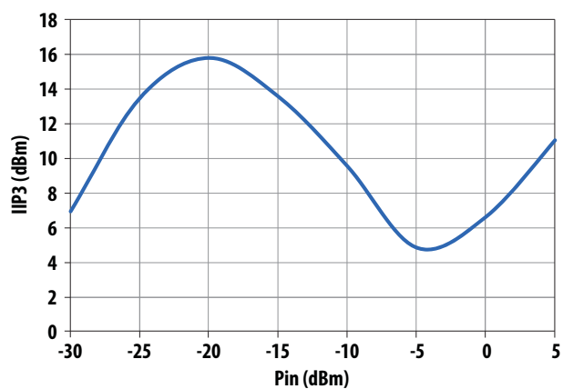
Figure 35. Bypass Mode IIP3 vs Input Power
