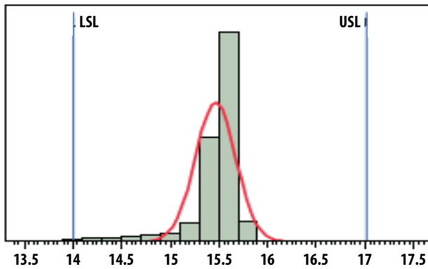
Figure 1. Gain @ 2.4 GHz, V_{dd} 3\text{ V} ; V_{bias} 1.8\text{ V} LSL = 14.3 dB, Nominal = 15.3 dB, USL = 16.7 dB
