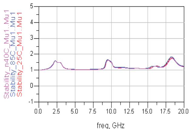
Figure 30. Edwards-Sinsky Output Stability Factor ( \mu ) at Vdd = 3 V
