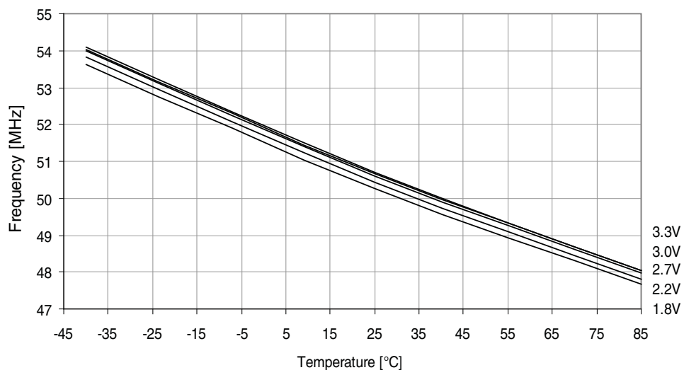
Figure 37-78. 48MHz internal oscillator frequency vs. temperature.
