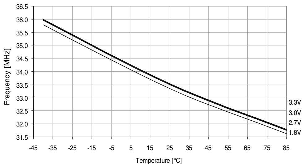
Figure 37-74. 32MHz internal oscillator frequency vs. temperature. DFLL disabled.
