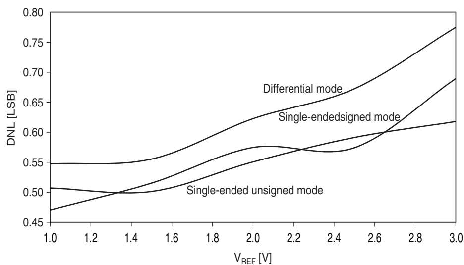
Figure 37-38. DNL error vs. external V_{REF} . T = 25^{\circ}\text{C} , V_{CC} = 3.6\text{V} , external reference.
