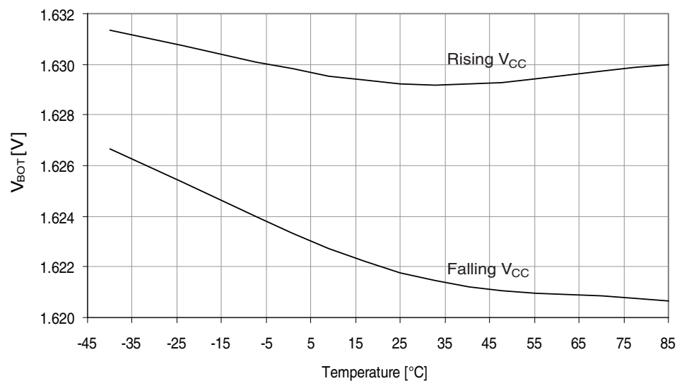
Figure 37-59. BOD thresholds vs. temperature.
