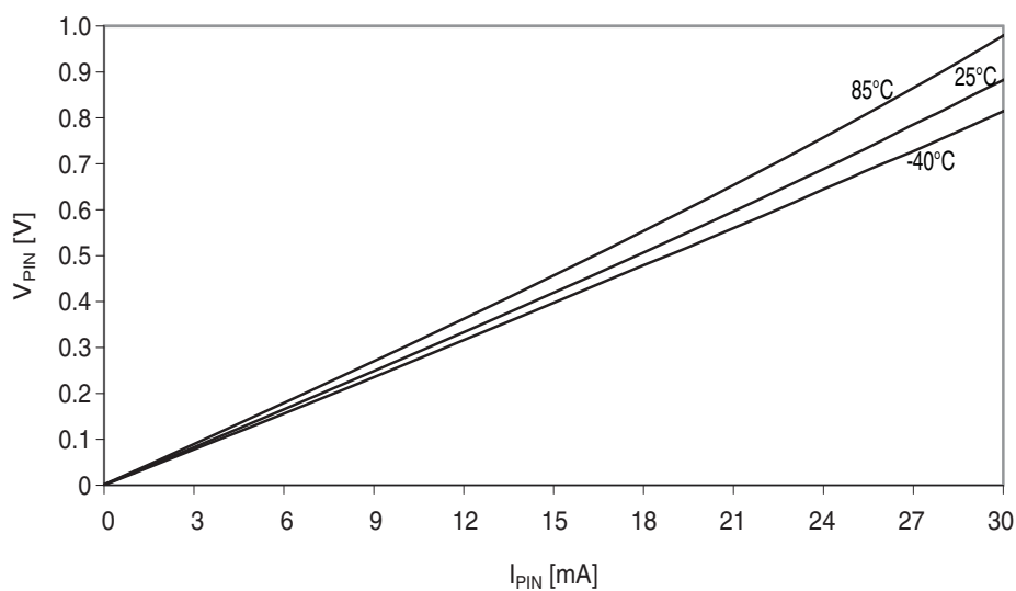
Figure 37-28. I/O pin output voltage vs. sink current. V_{CC} = 3.0V .
