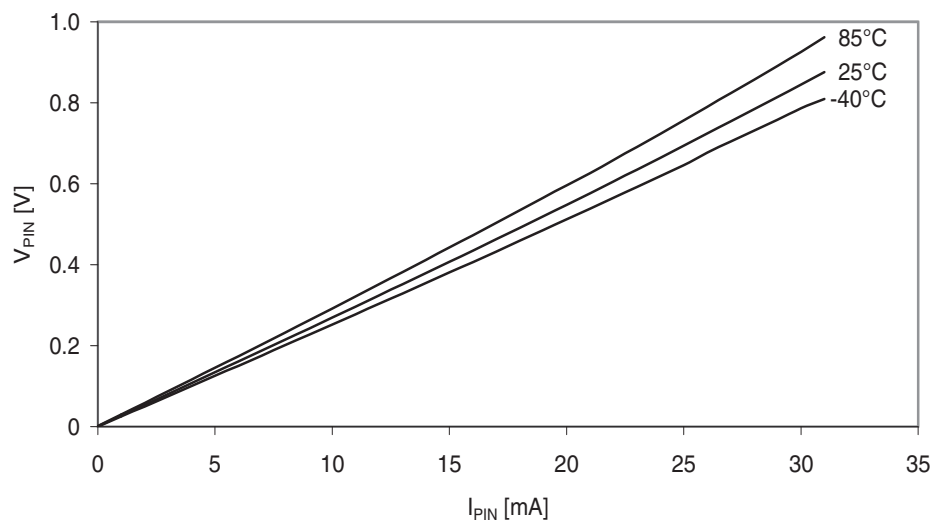
Figure 37-29. I/O pin output voltage vs. sink current. V_{CC} = 3.3V .
