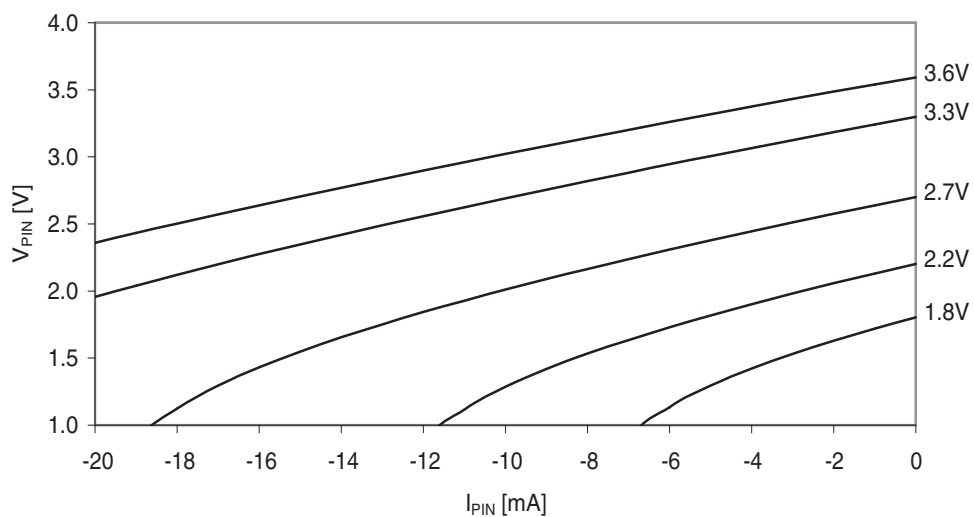
Figure 37-26. I/O pin output voltage vs. source current.
