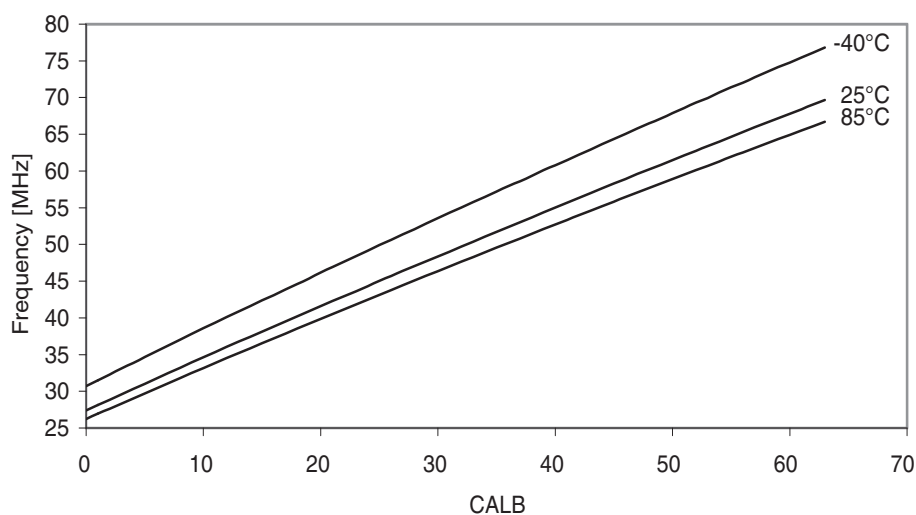
Figure 37-77. 32MHz internal oscillator frequency vs. CALB calibration value. V_{CC} = 3.0V .
