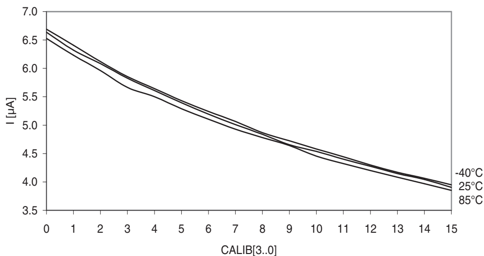
Figure 37-56. Analog comparator current source vs. calibration value. V CC = 3.0V.
