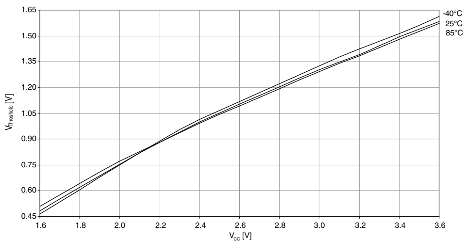
Figure 37-66. Reset pin input threshold voltage vs. V_{CC} .
