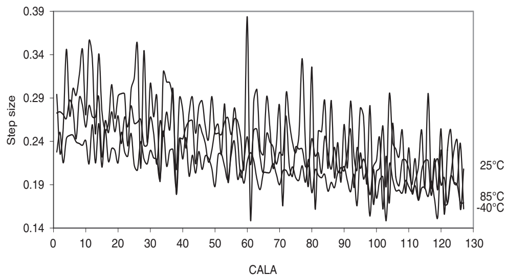
Figure 37-76. 32MHz internal oscillator CALA calibration step size. V_{CC} = 3.0V .
