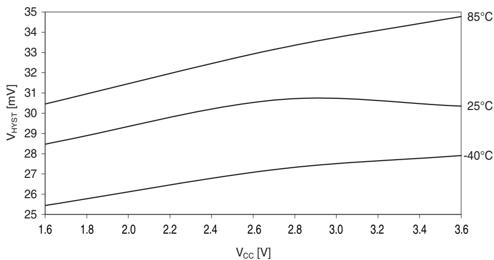
Figure 37-52. Analog comparator hysteresis vs. V_{CC} .
