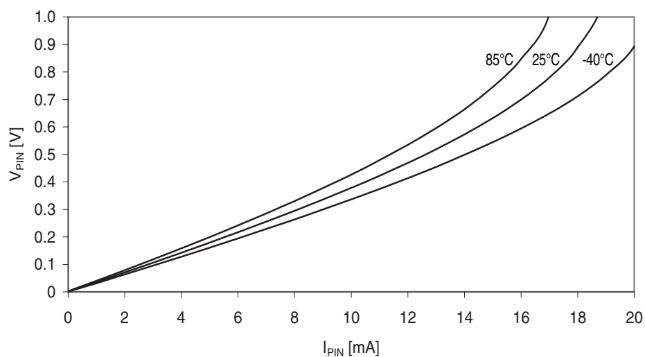
Figure 37-27. I/O pin output voltage vs. sink current. V_{CC} = 1.8V .
