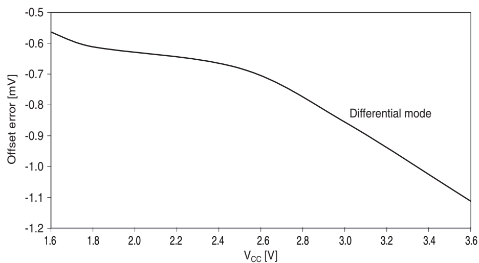
Figure 37-45. Offset error vs. V_{CC} .
