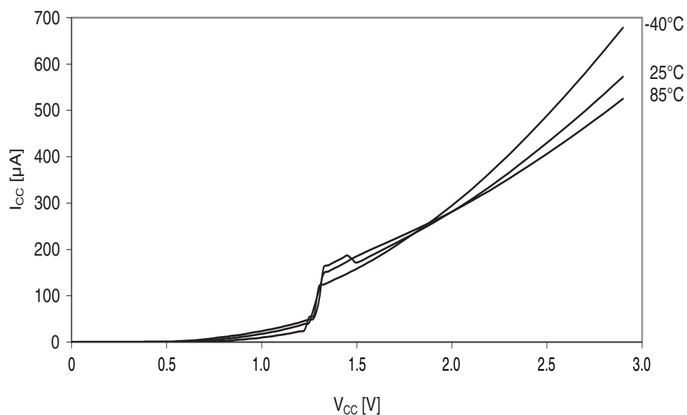
Figure 37-67. Power-on reset current consumption vs. V_{CC} .
