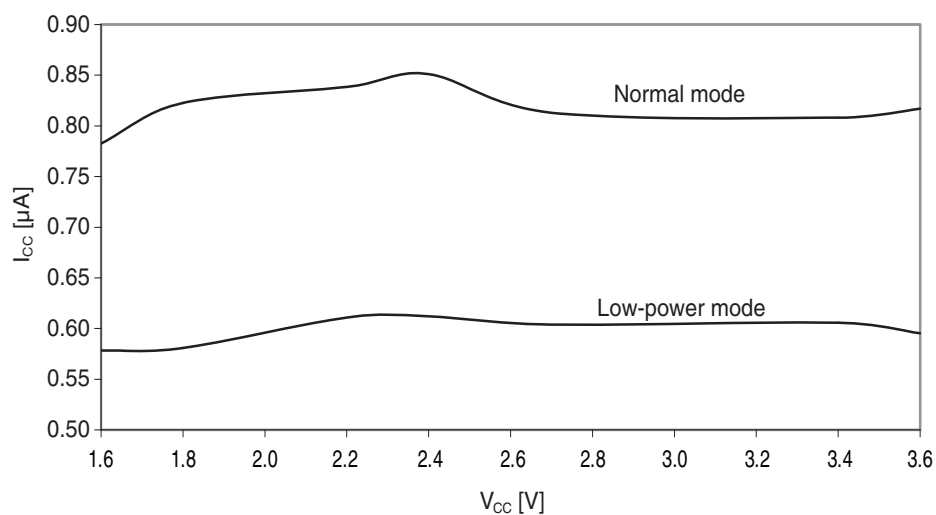
Figure 37-17. Power-save mode supply current vs. V_{CC} .
