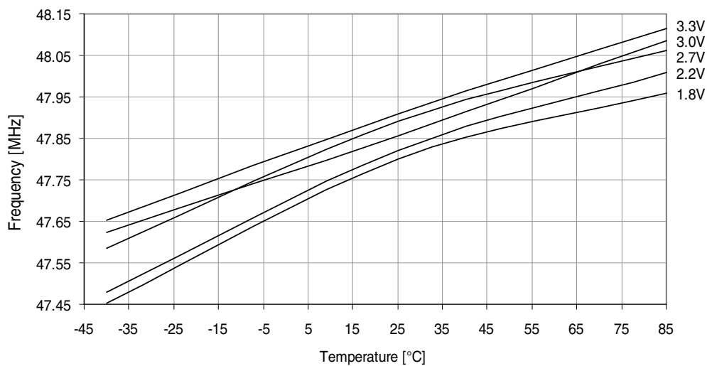
Figure 37-79. 48MHz internal oscillator frequency vs. temperature.
