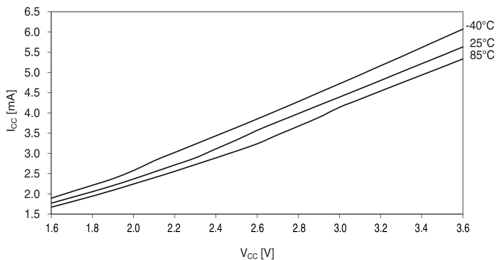
Figure 37-6. Active mode supply current vs. V_{CC} .
