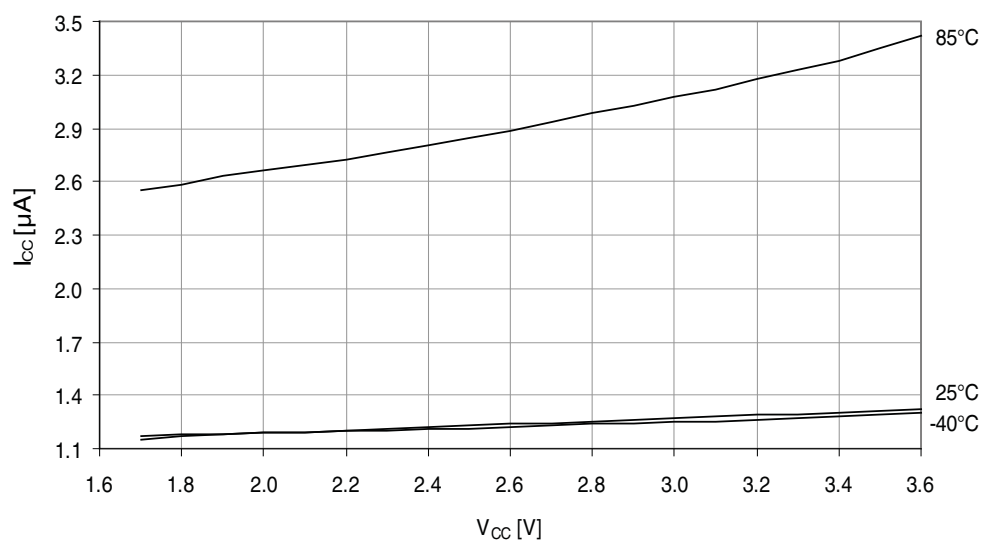
Figure 37-16. Power-down mode supply current vs. V_{CC} . Watchdog and sampled BOD enabled.
