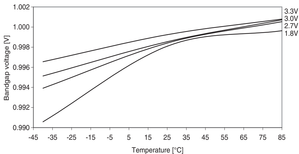
Figure 37-58. ADC/DAC Internal 1.0V reference vs. temperature.
