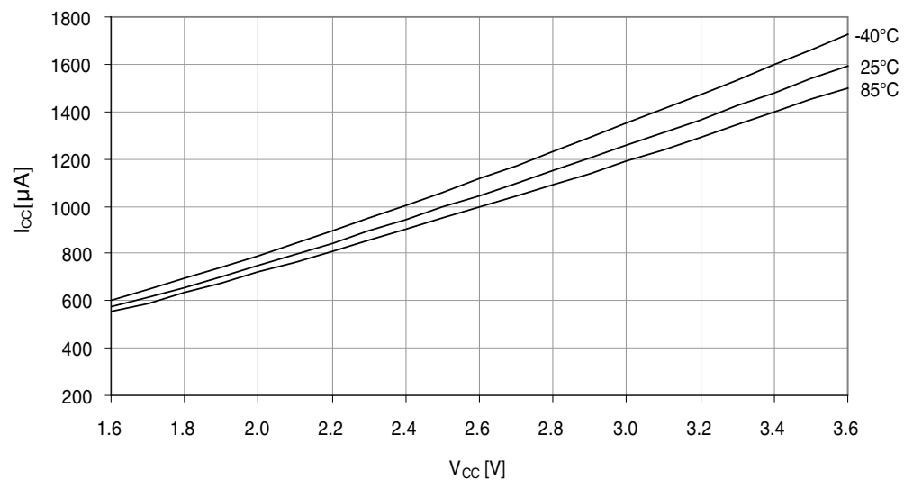
Figure 37-5. Active mode supply current vs. V_{CC} .
