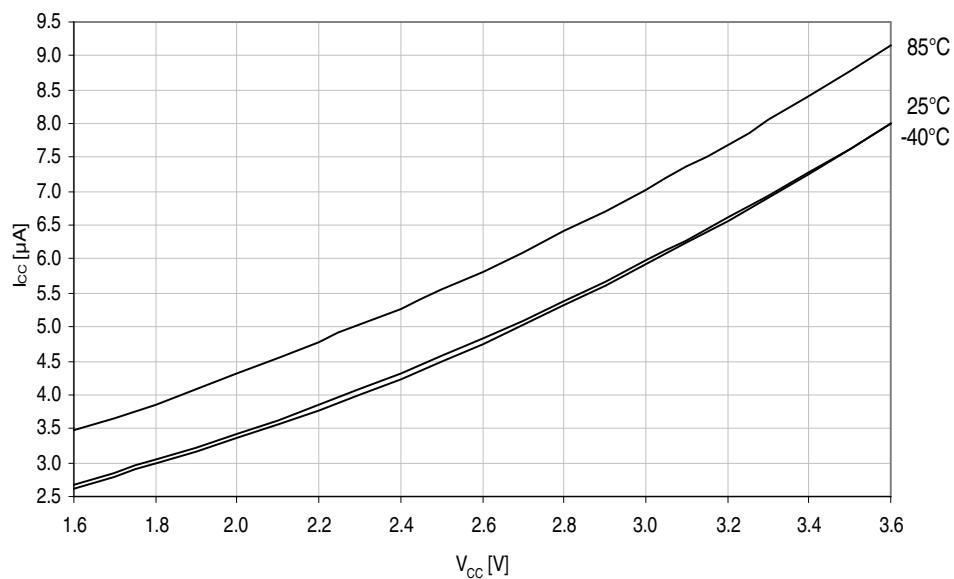
Figure 37-18. Standby supply current vs. V_{CC} .
