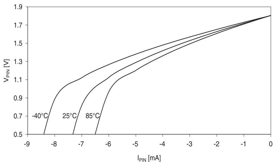
Figure 37-23. I/O pin output voltage vs. source current. V_{CC} = 1.8V .
