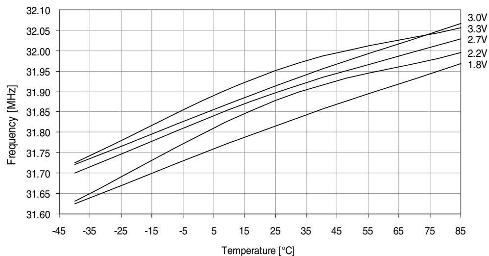
Figure 37-75. 32MHz internal oscillator frequency vs. temperature. DFLL enabled, from the 32.768kHz internal oscillator.
