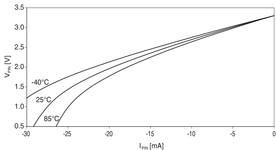
Figure 37-25. I/O pin output voltage vs. source current. V_{CC} = 3.3V .
