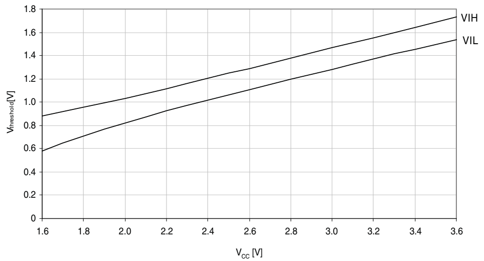
Figure 37-32. I/O pin input threshold voltage vs. V_{CC} . T = 25^{\circ}C .
