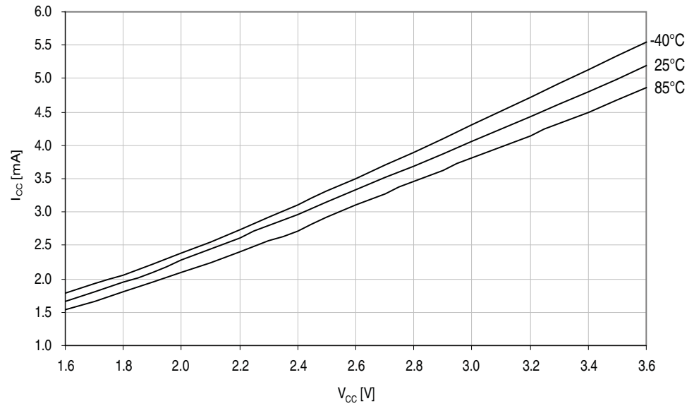
Figure 37-6. Active mode supply current vs. V_{CC} . f_{SYS} = 32MHz internal oscillator prescaled to 8MHz.
