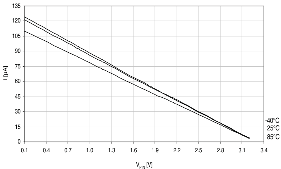
Figure 37-23. I/O pin pull-up resistor current vs. input voltage.
