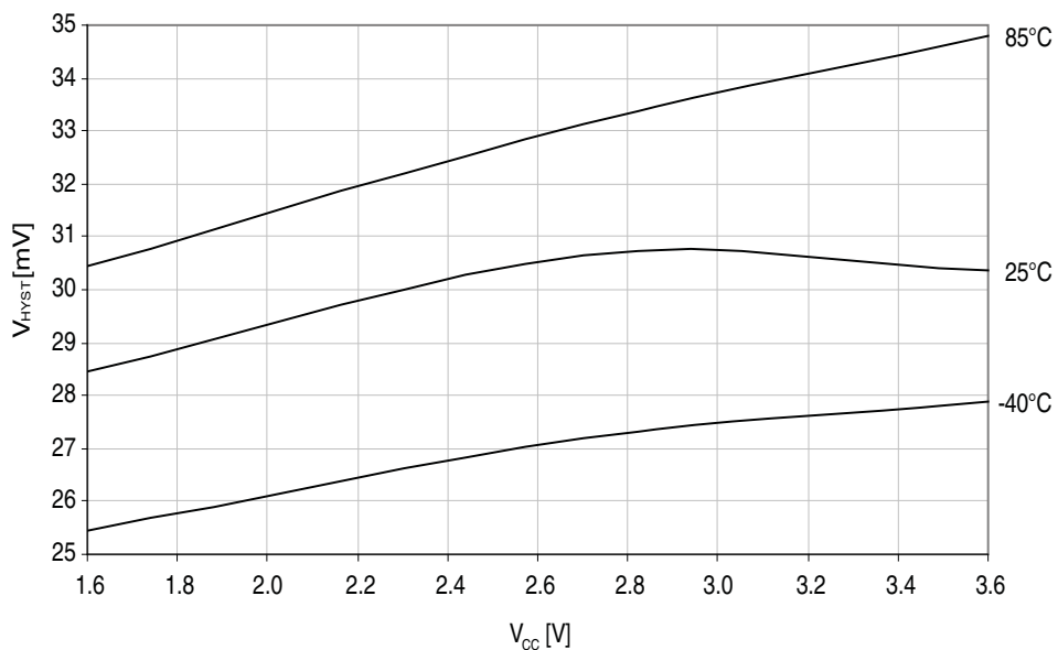
Figure 37-53. Analog comparator hysteresis vs. V_{CC} . Low power, small hysteresis.
