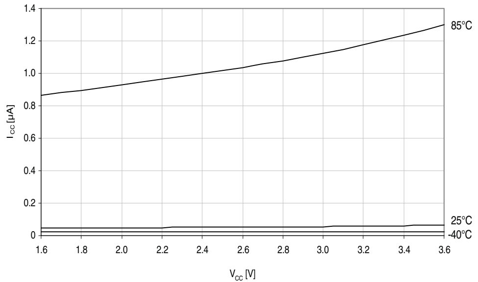
Figure 37-16. Power-down mode supply current vs. V_{CC} . All functions disabled.
