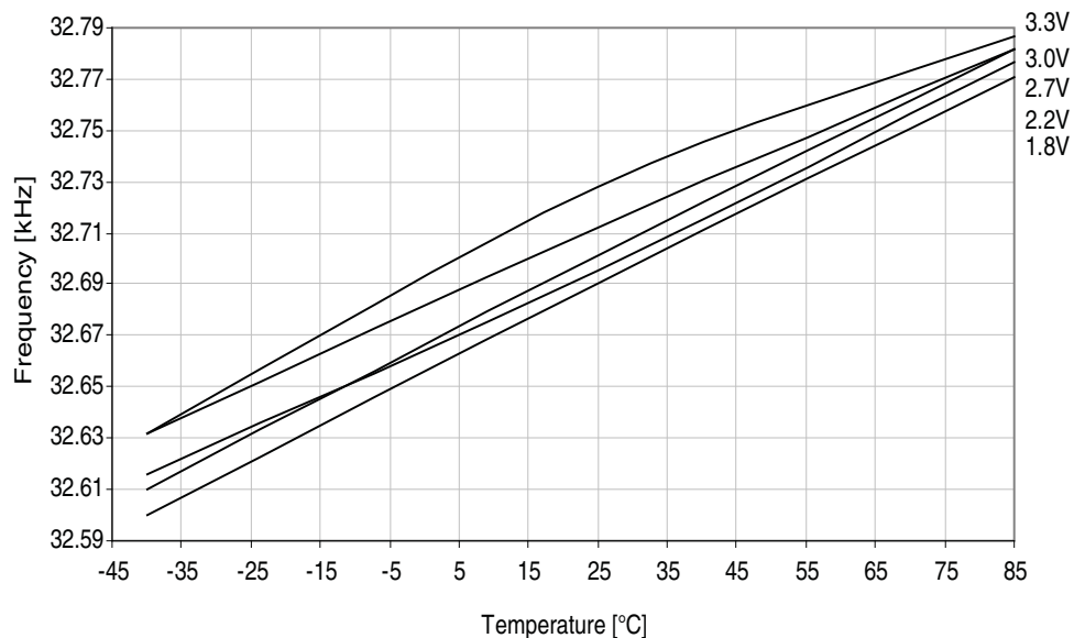
Figure 37-71. 32.768kHz internal oscillator frequency vs. temperature.
