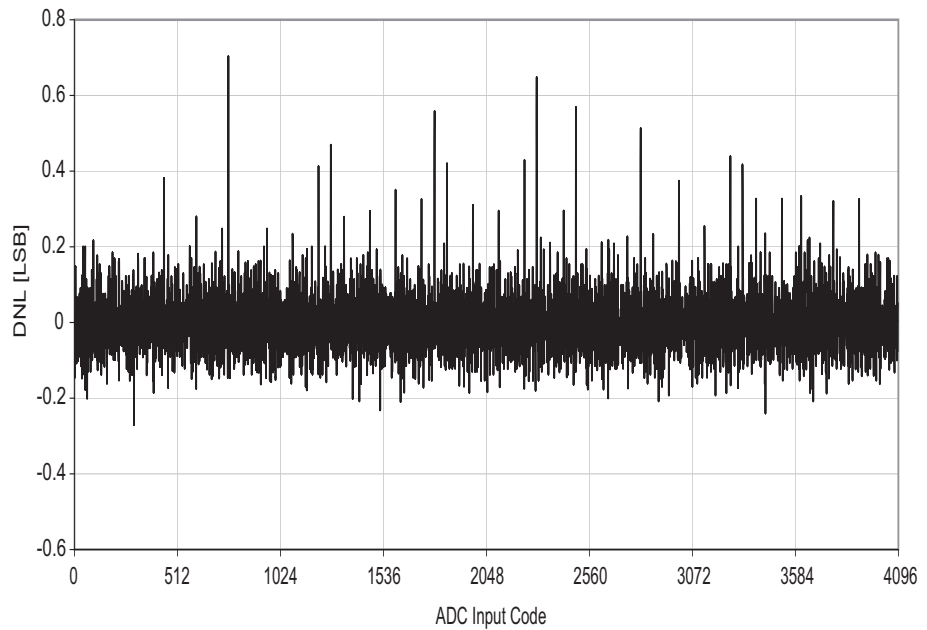
Figure 37-41. DNL error vs. input code.
