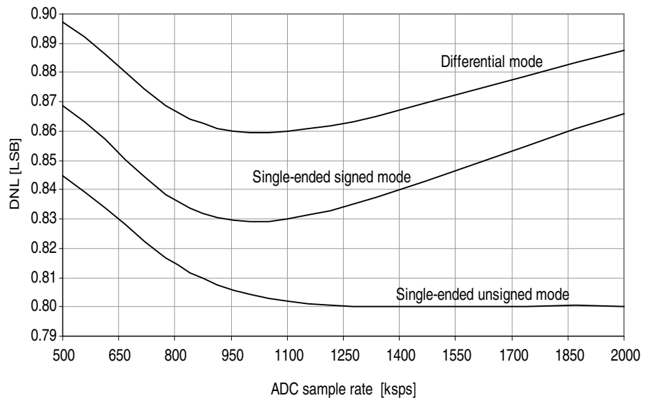
Figure 37-40. DNL error vs. sample rate.
