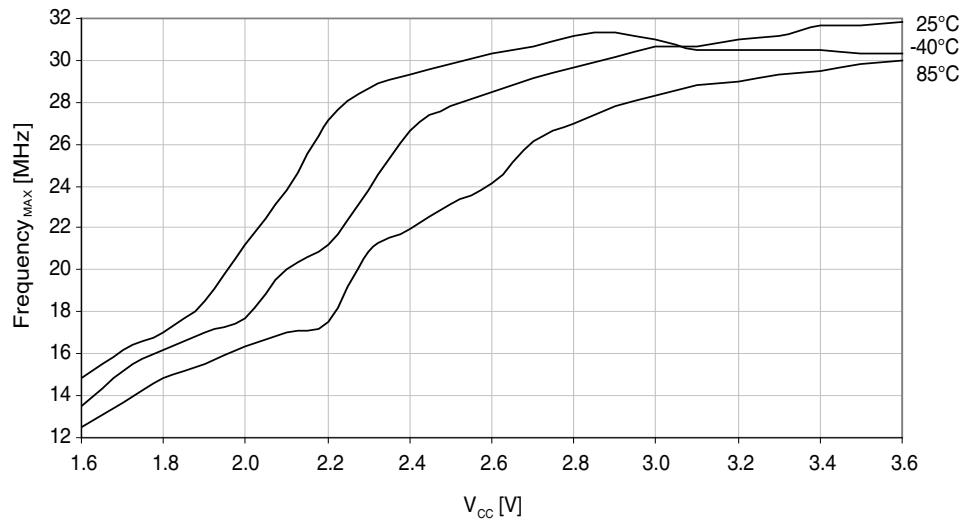
Figure 37-85. Maximum PDI frequency vs. V CC .
