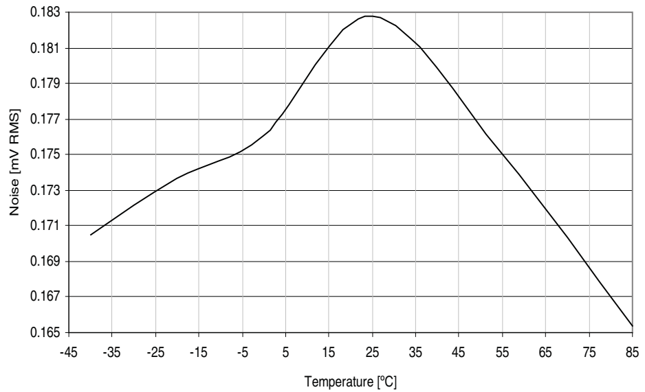
Figure 37-51. DAC noise vs. temperature.
