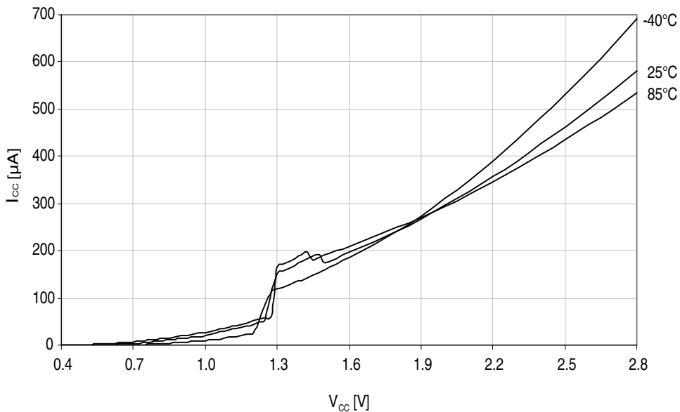
Figure 37-68. Power-on reset current consumption vs. V_{CC} . BOD level = 3.0V, enabled in continuous mode.
