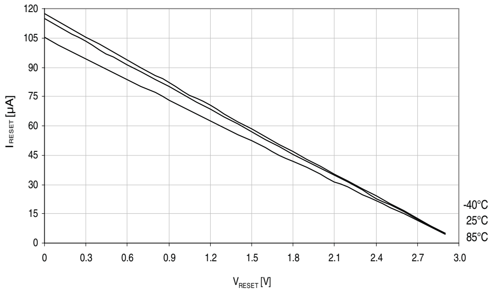
Figure 37-64. Reset pin pull-up resistor current vs. reset pin voltage.
