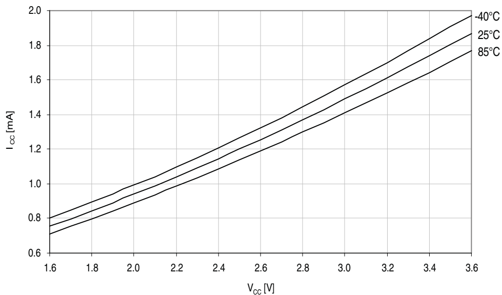
Figure 37-14. Idle mode current vs. V_{CC} . f_{SYS} = 32MHz internal oscillator.
