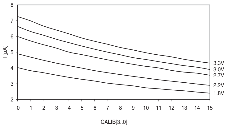
Figure 37-56. Analog comparator current source vs. calibration value. Temperature = 25°C.
