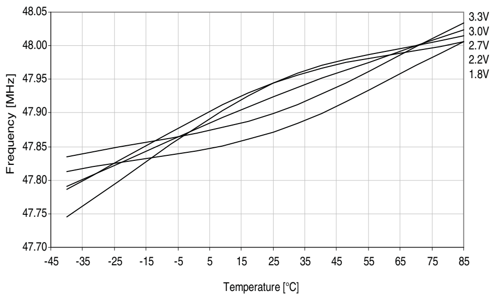
Figure 37-81. 48MHz internal oscillator frequency vs. temperature. DPLL enabled, from the 32.768kHz internal oscillator.
