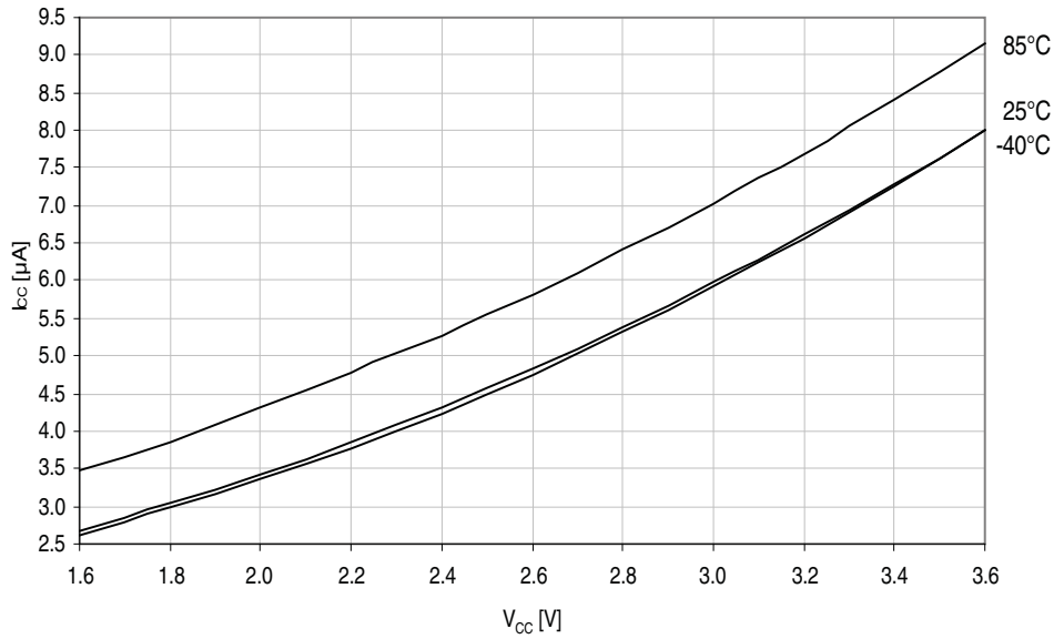
Figure 37-19. Standby supply current vs. V_{CC} . Standby, f_{SYS} = 1\text{MHz} .
