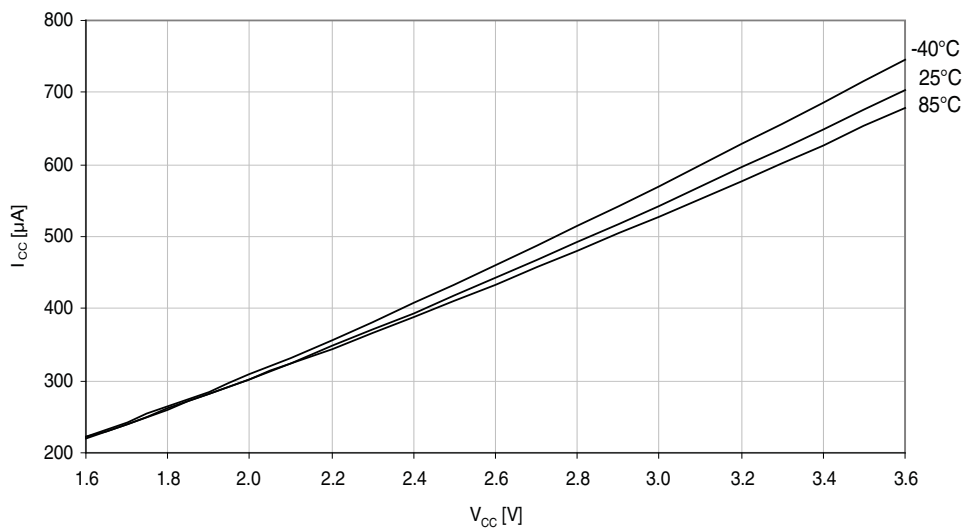
Figure 37-4. Active mode supply current vs. V_{CC} .
