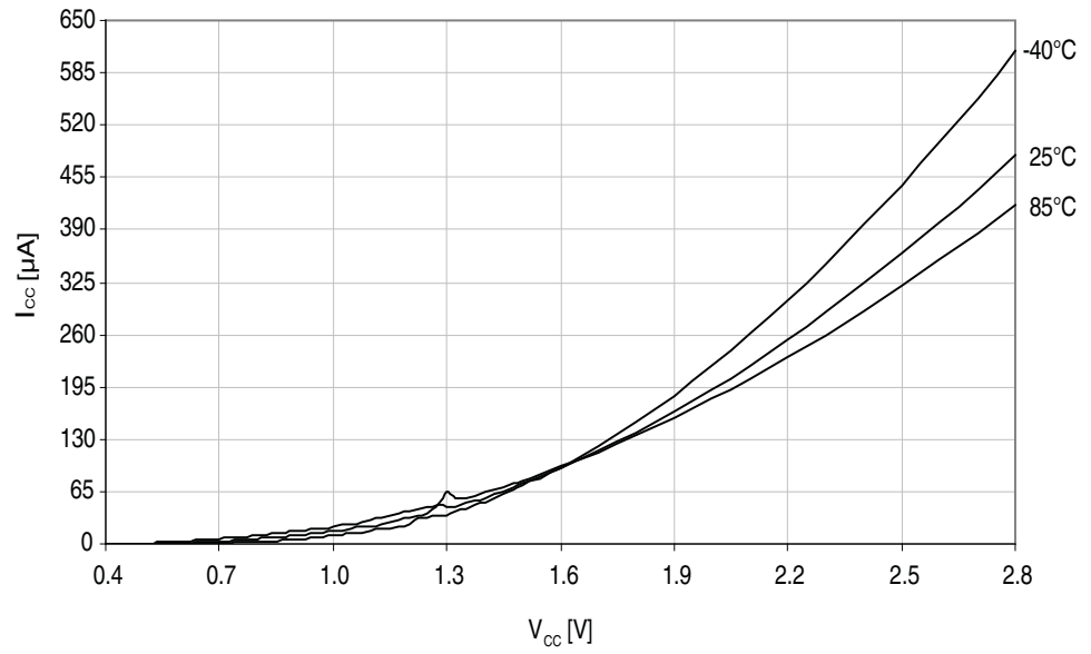
Figure 37-69. Power-on reset current consumption vs. V_{CC} . BOD level = 3.0V, enabled in sampled mode.
