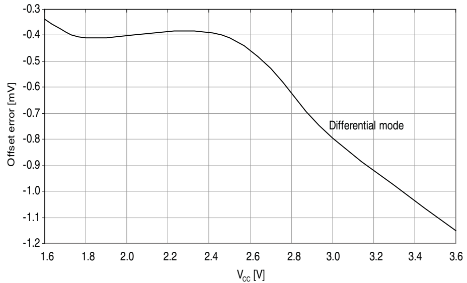
Figure 37-46. Offset error vs. V_{CC} .
