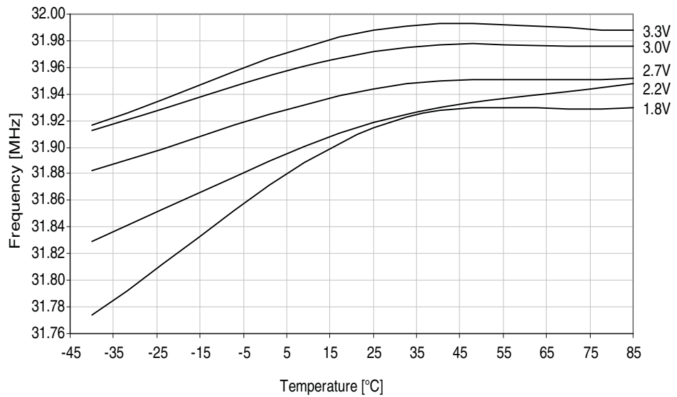
Figure 37-77. 32MHz internal oscillator frequency vs. temperature.
