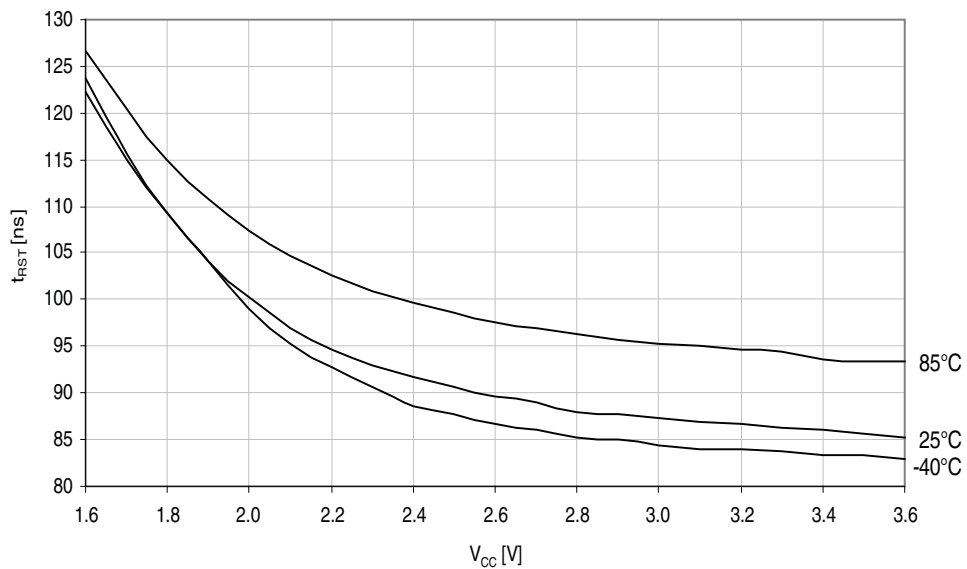
Figure 37-62. Minimum Reset pin pulse width vs. V_{CC} .
