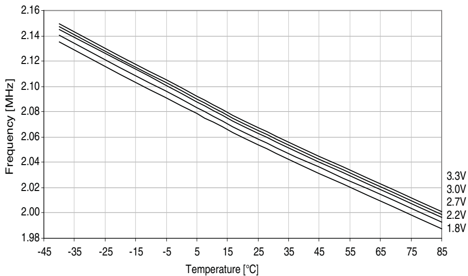
Figure 37-73. 2MHz internal oscillator frequency vs. temperature.
