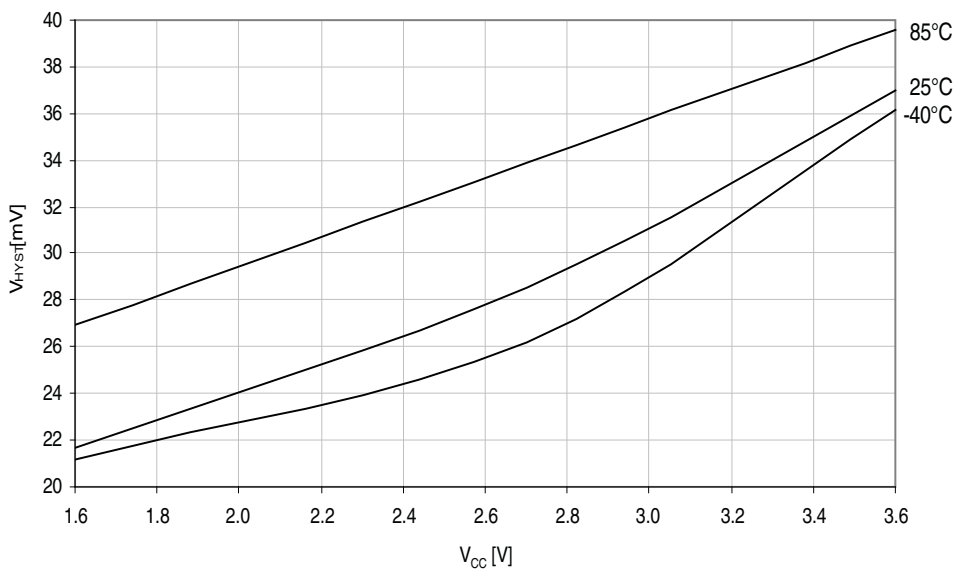
Figure 37-54. Analog comparator hysteresis vs. V_{CC} . High-speed mode, large hysteresis.
