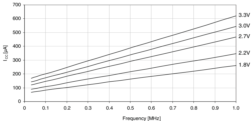
Figure 37-2. Active supply current vs. frequency.
