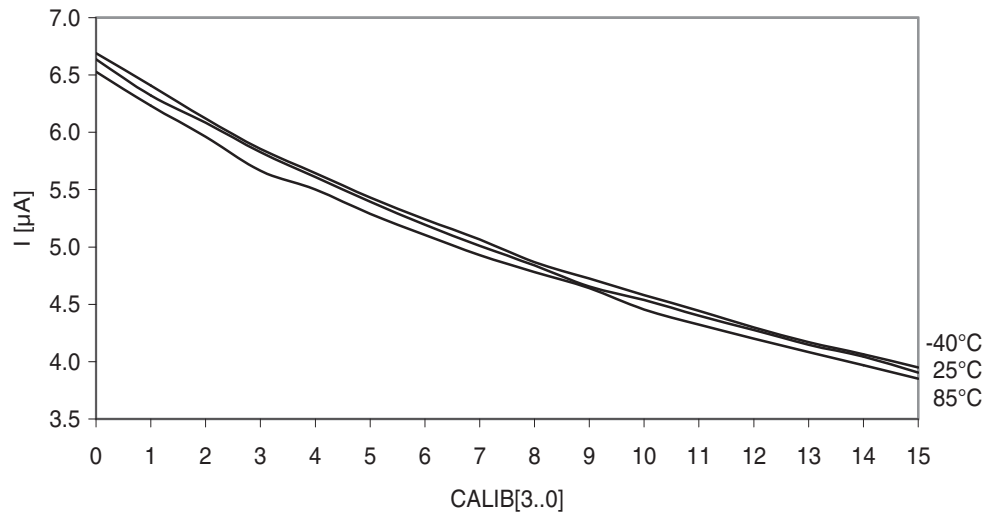
Figure 37-57. Analog comparator current source vs. calibration value.
