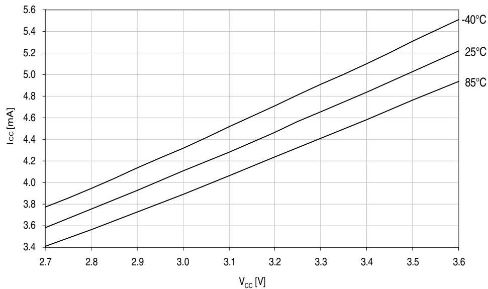
Figure 37-14. Idle mode current vs. V_{CC} . f_{SYS} = 32MHz internal oscillator.
