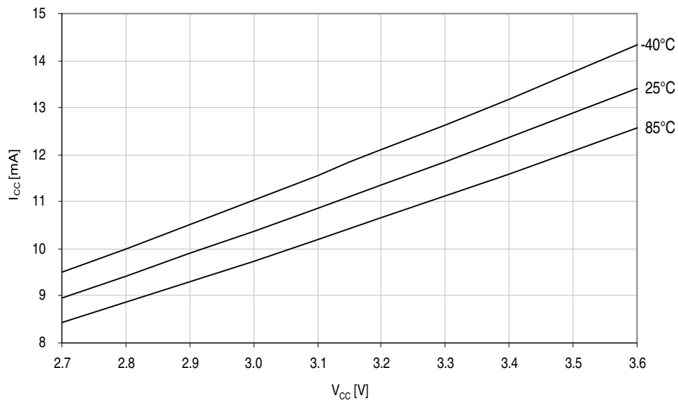
Figure 37-7. Active mode supply current vs. V_{CC} . f_{SYS} = 32\text{MHz} internal oscillator.
