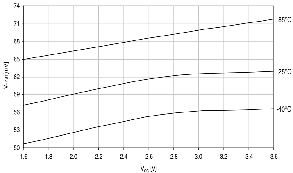
Figure 37-55. Analog comparator hysteresis vs. V_{CC} . Low power, large hysteresis.
