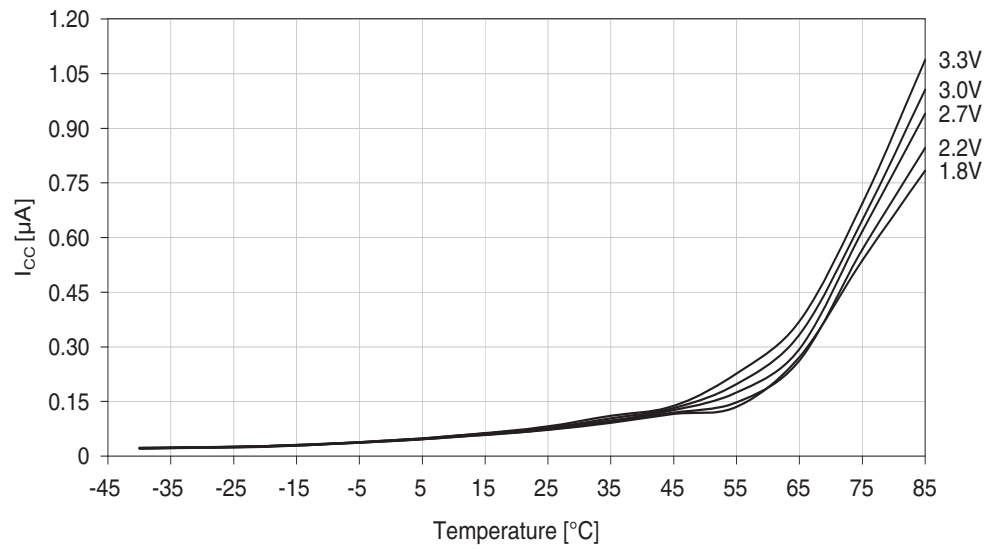
Figure 37-15. Power-down mode supply current vs. temperature. All functions disabled.
