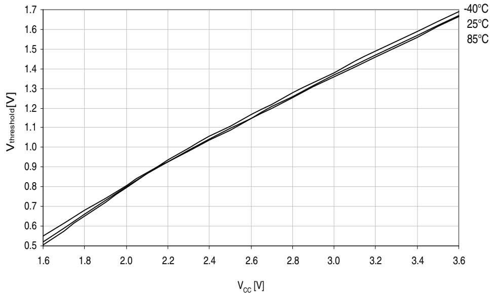
Figure 37-67. Reset pin input threshold voltage vs. V_{CC} . V_{IL} - Reset pin read as "0".
