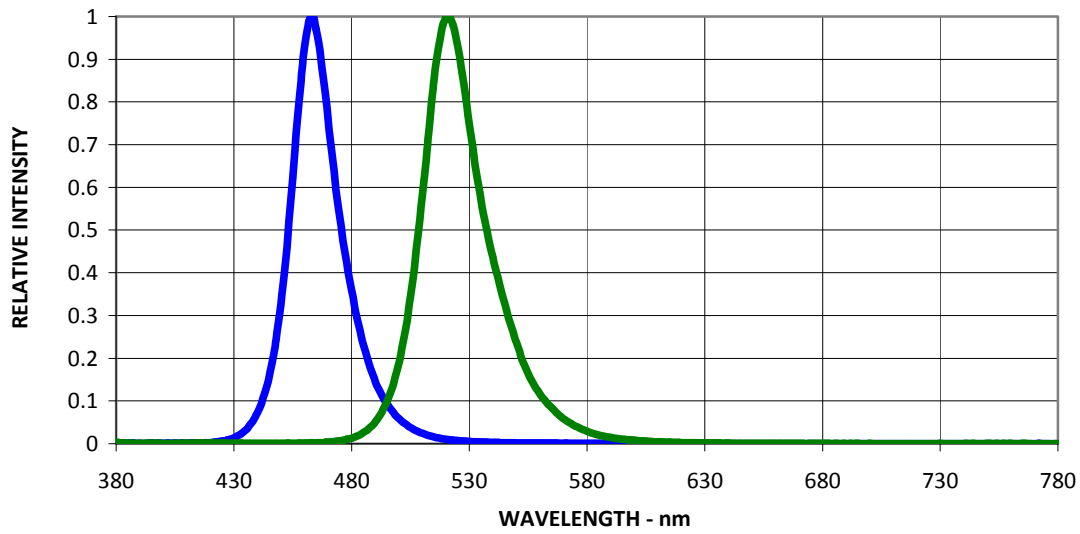
Figure 1. Relative Intensity Vs. Wavelength (ASMT-SBB5 and ASMT-SGB5)
