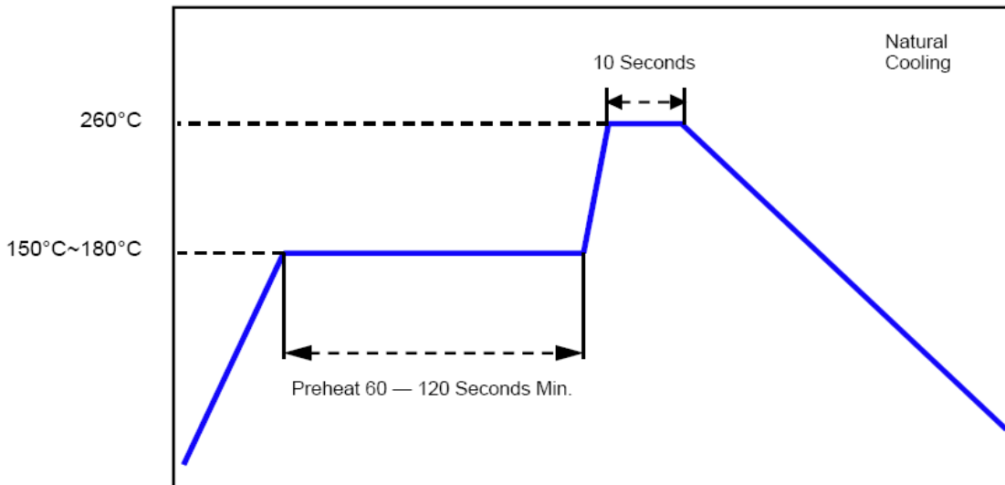
Recommended Temperature Profile for Lead-free Solder
