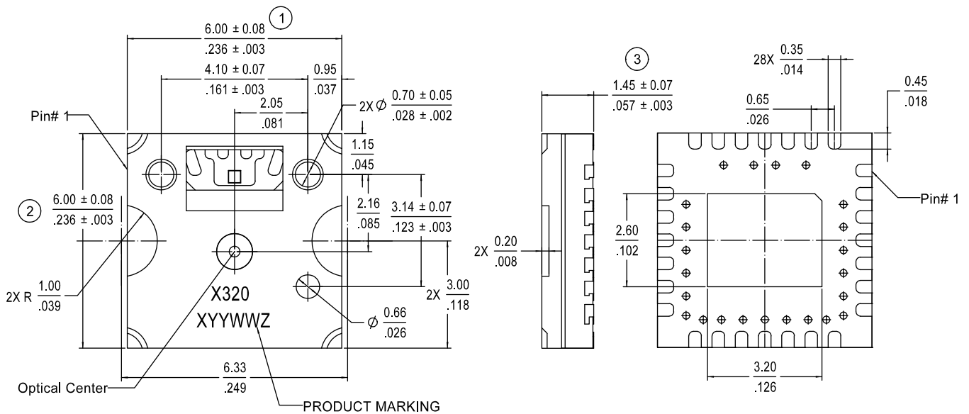
Figure 1b. Package outline drawing (top view)
