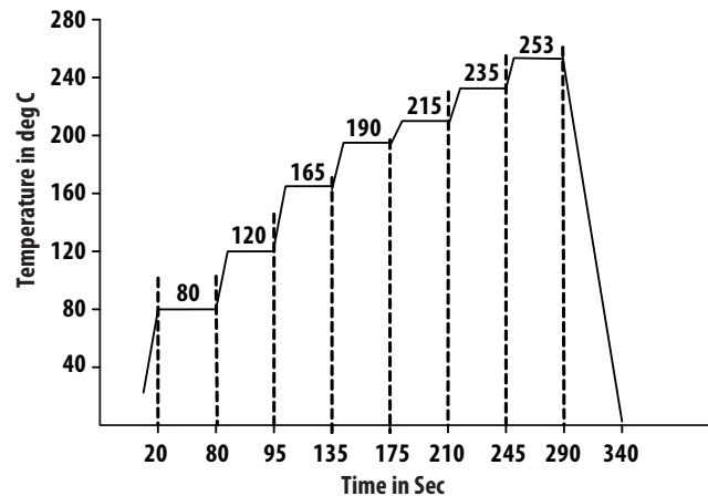
Figure 3a. Recommended reflow profile
