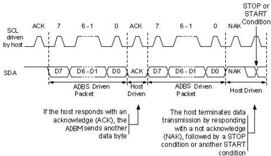
Figure 19. Sensor packets
