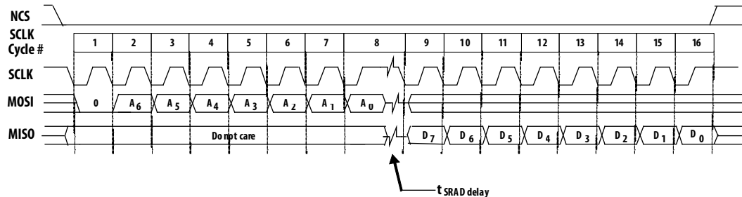
Figure 11. Read Operation
