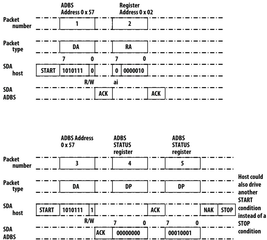
Figure 22. TWI polling
