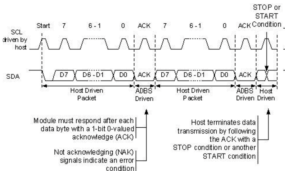
Figure 18. Host packets
