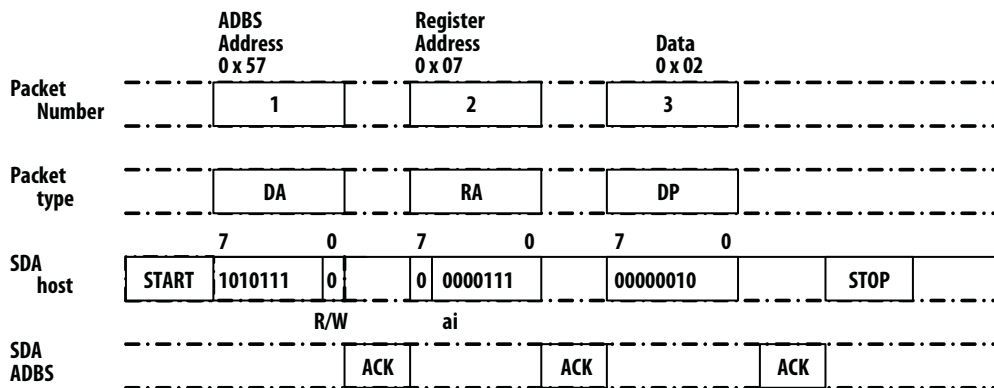
Figure 20. TWI write
