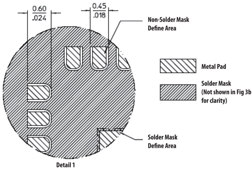
Figure 3c. Recommended Customer's PCB PADOUT and spacing
