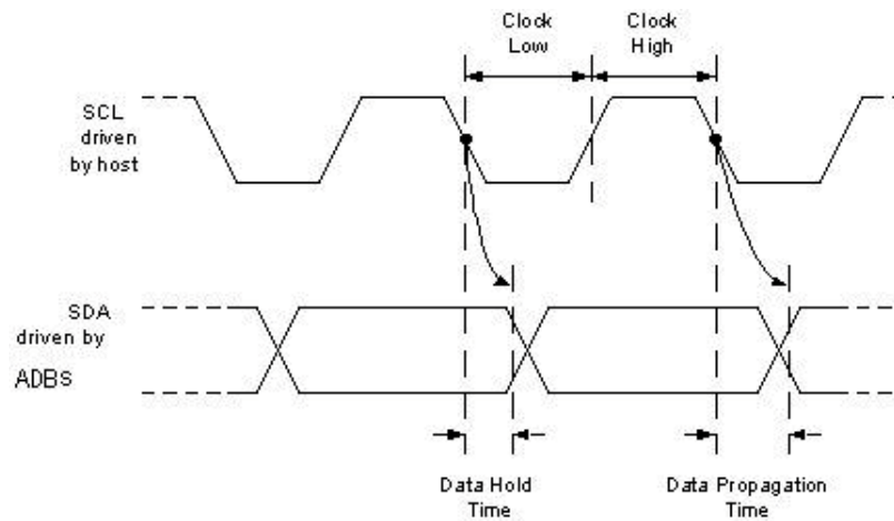
Figure 24. TWI SCL and SDA Timing
