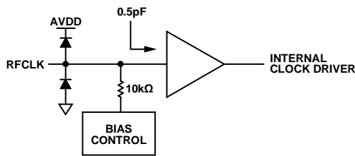
Figure 29. Equivalent RF Clock Input Circuit
