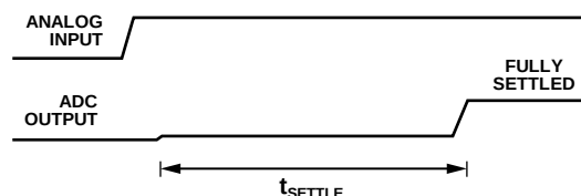
Figure 38. Step Input with Single Cycle Settling
