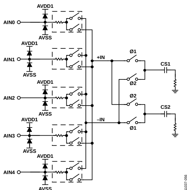
Figure 29. Simplified Analog Input Circuit
